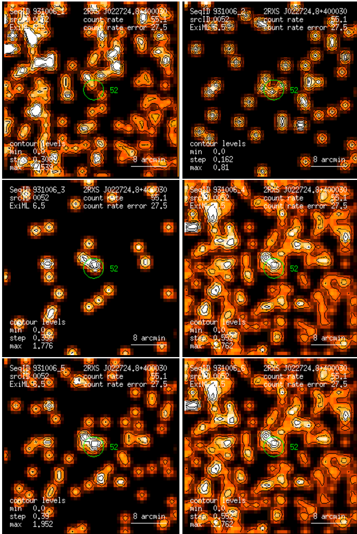
Figure 52: RASS 931006: detection 0052: band rate images, Gaussian filter: (1) PSPC channels 11 – 41, (2) 52 – 90, (3) 91 – 201, (4) 11 – 235, (5) 52 – 201, (6) 11 – 201. Broad band rates in counts/ks. Band rate contour levels in counts/ks/arcmin 2 .
