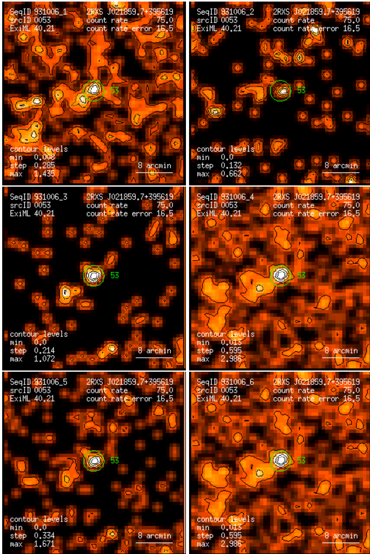
Figure 53: RASS 931006: detection 0053: band rate images, Gaussian filter: (1) PSPC channels 11 – 41, (2) 52 – 90, (3) 91 – 201, (4) 11 – 235, (5) 52 – 201, (6) 11 – 201. Broad band rates in counts/ks. Band rate contour levels in counts/ks/arcmin 2 .
