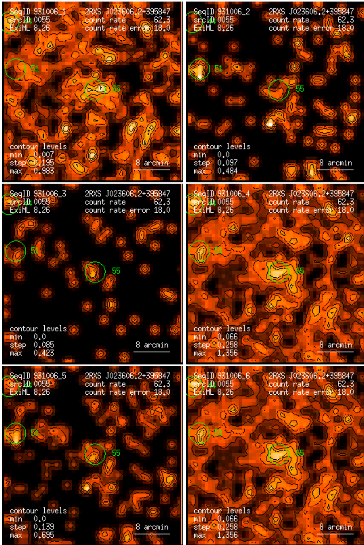
Figure 55: RASS 931006: detection 0055: band rate images, Gaussian filter: (1) PSPC channels 11 – 41, (2) 52 – 90, (3) 91 – 201, (4) 11 – 235, (5) 52 – 201, (6) 11 – 201. Broad band rates in counts/ks. Band rate contour levels in counts/ks/arcmin 2 .
