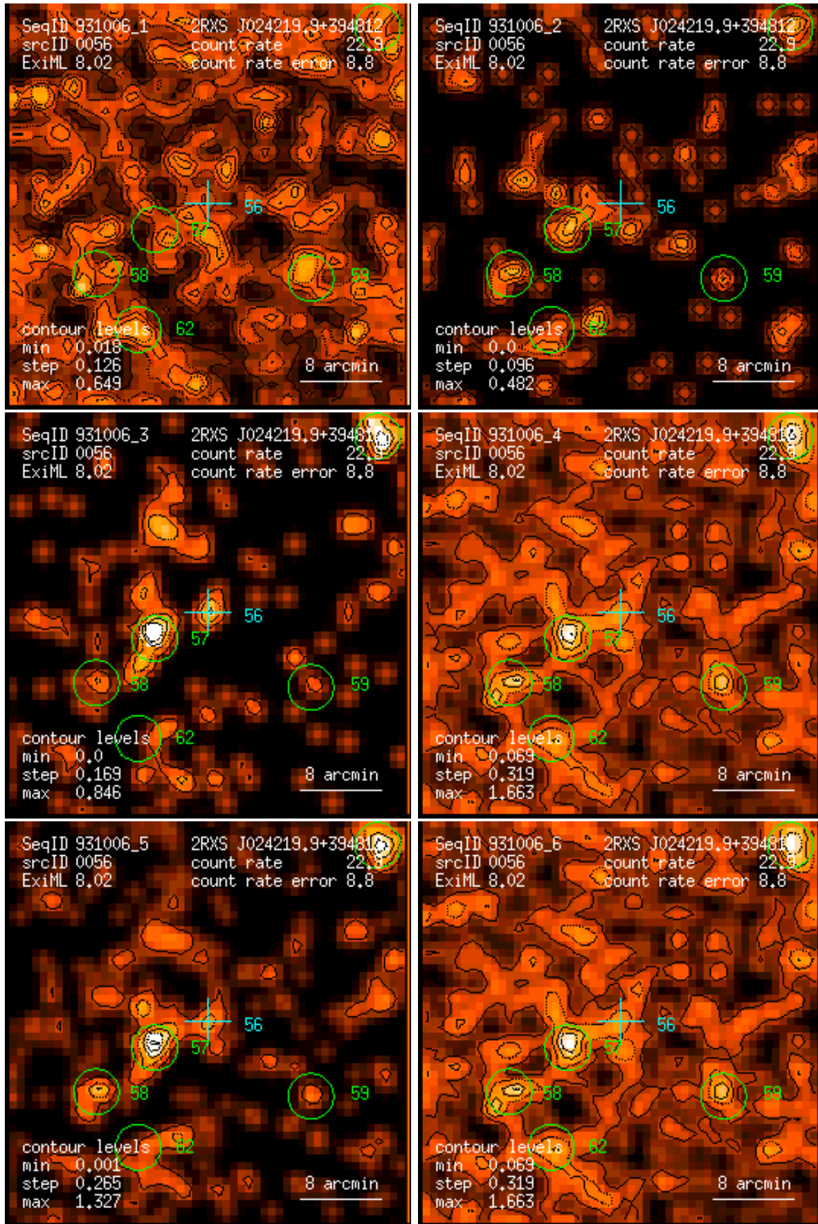
Figure 56: RASS 931006: detection 0056: band rate images, Gaussian filter: (1) PSPC channels 11 – 41, (2) 52 – 90, (3) 91 – 201, (4) 11 – 235, (5) 52 – 201, (6) 11 – 201. Broad band rates in counts/ks. Band rate contour levels in counts/ks/arcmin 2 .
