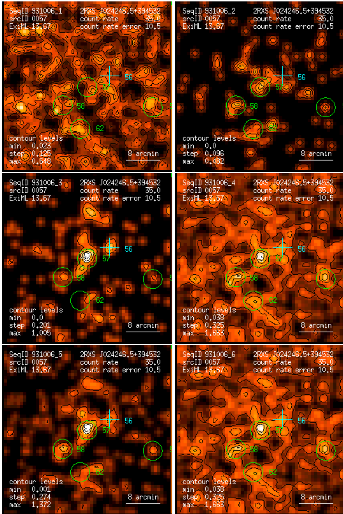
Figure 57: RASS 931006: detection 0057: band rate images, Gaussian filter: (1) PSPC channels 11 – 41, (2) 52 – 90, (3) 91 – 201, (4) 11 – 235, (5) 52 – 201, (6) 11 – 201. Broad band rates in counts/ks. Band rate contour levels in counts/ks/arcmin 2 .
