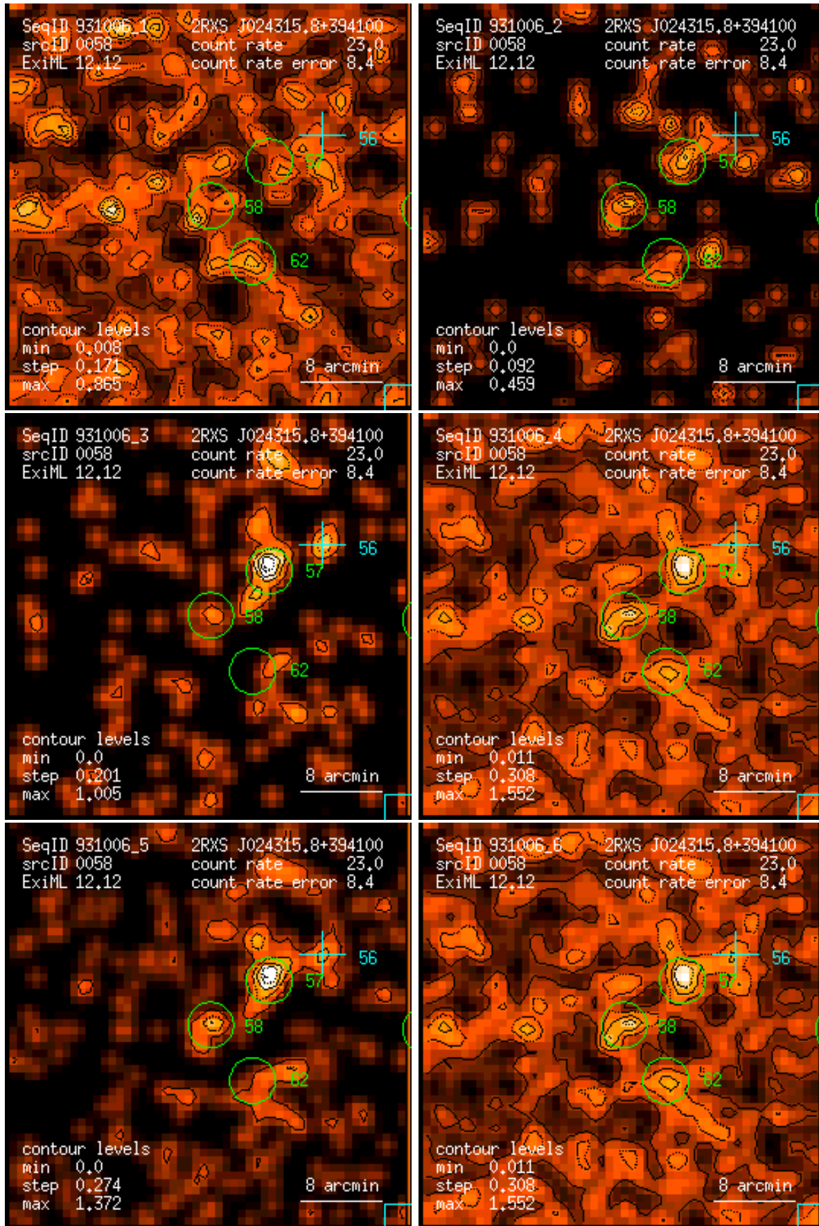
Figure 58: RASS 931006: detection 0058: band rate images, Gaussian filter: (1) PSPC channels 11 – 41, (2) 52 – 90, (3) 91 – 201, (4) 11 – 235, (5) 52 – 201, (6) 11 – 201. Broad band rates in counts/ks. Band rate contour levels in counts/ks/arcmin 2 .
