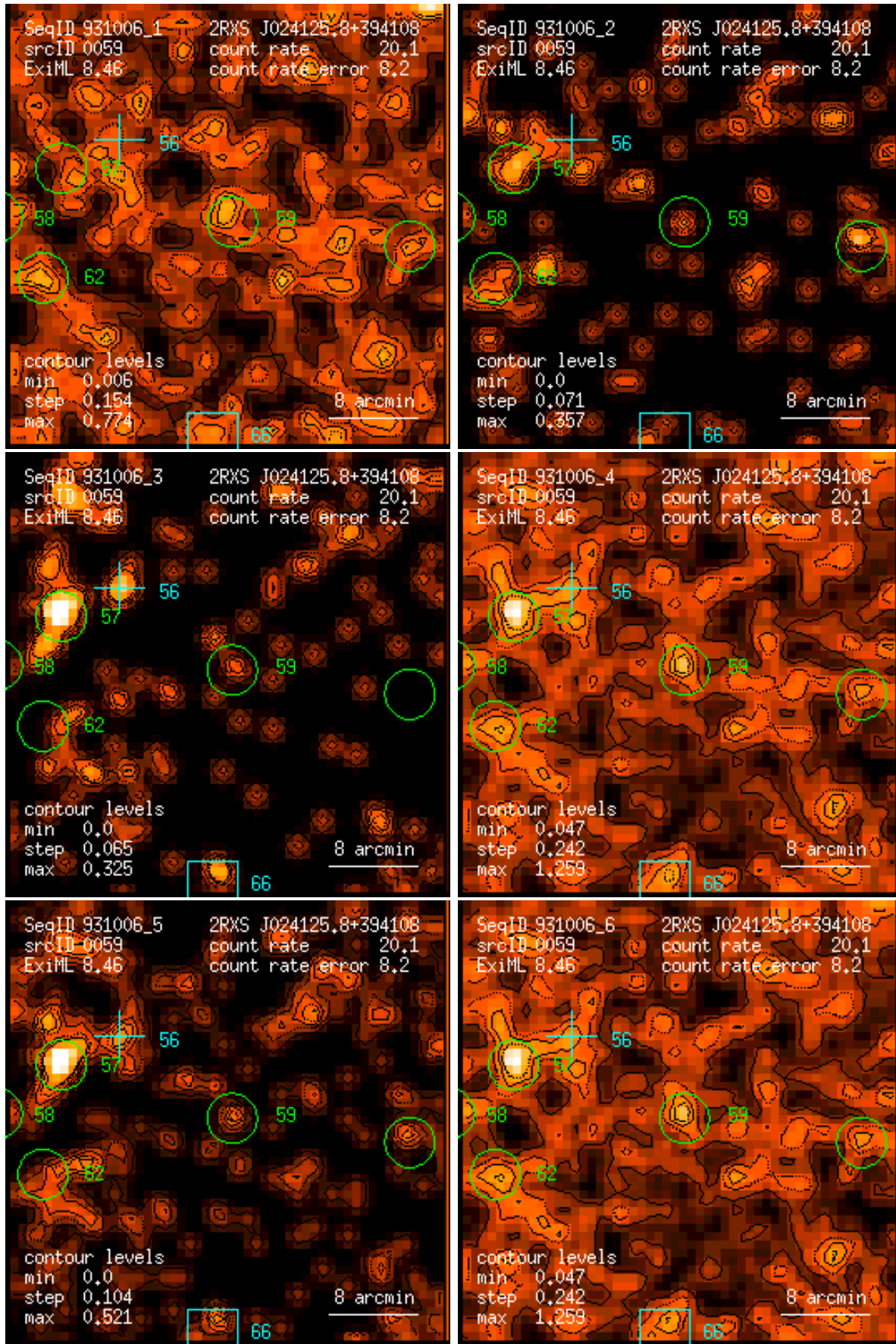
Figure 59: RASS 931006: detection 0059: band rate images, Gaussian filter: (1) PSPC channels 11 – 41, (2) 52 – 90, (3) 91 – 201, (4) 11 – 235, (5) 52 – 201, (6) 11 – 201. Broad band rates in counts/ks. Band rate contour levels in counts/ks/arcmin 2 .
