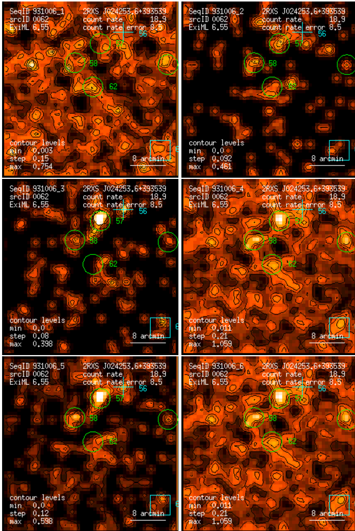
Figure 62: RASS 931006: detection 0062: band rate images, Gaussian filter: (1) PSPC channels 11 – 41, (2) 52 – 90, (3) 91 – 201, (4) 11 – 235, (5) 52 – 201, (6) 11 – 201. Broad band rates in counts/ks. Band rate contour levels in counts/ks/arcmin 2 .
