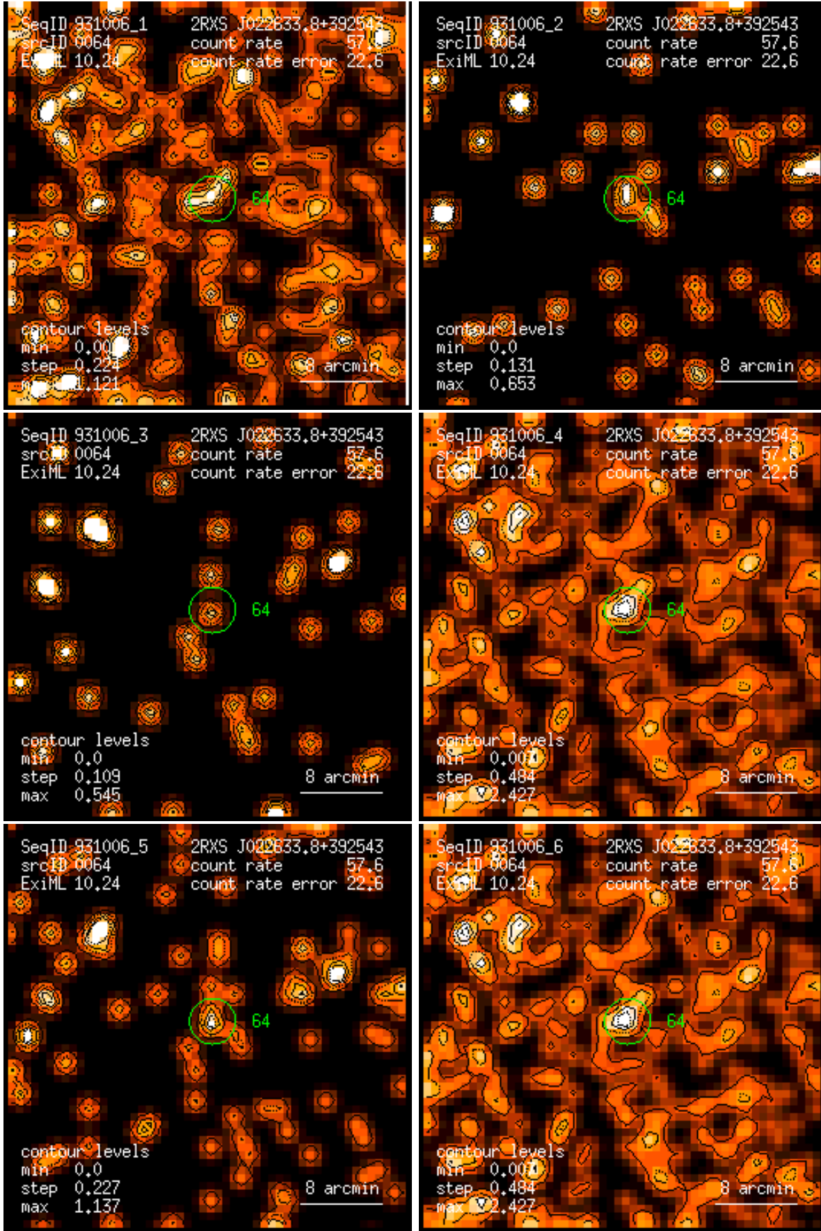
Figure 64: RASS 931006: detection 0064: band rate images, Gaussian filter: (1) PSPC channels 11 – 41, (2) 52 – 90, (3) 91 – 201, (4) 11 – 235, (5) 52 – 201, (6) 11 – 201. Broad band rates in counts/ks. Band rate contour levels in counts/ks/arcmin 2 .
