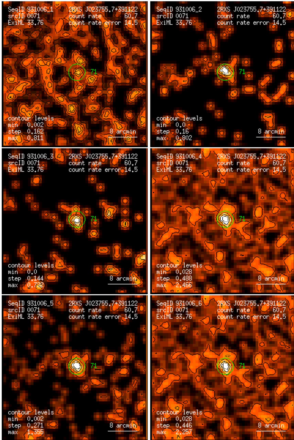
Figure 71: RASS 931006: detection 0071: band rate images, Gaussian filter: (1) PSPC channels 11 – 41, (2) 52 – 90, (3) 91 – 201, (4) 11 – 235, (5) 52 – 201, (6) 11 – 201. Broad band rates in counts/ks. Band rate contour levels in counts/ks/arcmin 2 .
