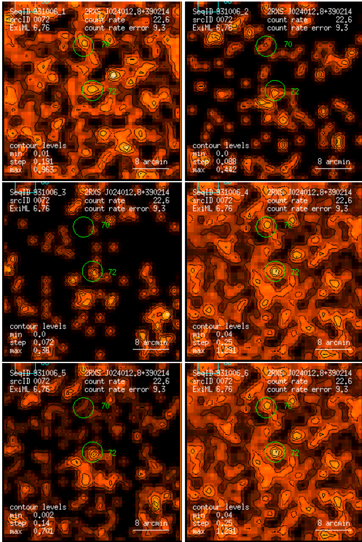
Figure 72: RASS 931006: detection 0072: band rate images, Gaussian filter: (1) PSPC channels 11 – 41, (2) 52 – 90, (3) 91 – 201, (4) 11 – 235, (5) 52 – 201, (6) 11 – 201. Broad band rates in counts/ks. Band rate contour levels in counts/ks/arcmin 2 .
