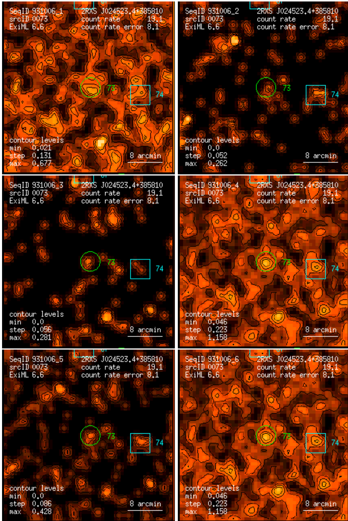
Figure 73: RASS 931006: detection 0073: band rate images, Gaussian filter: (1) PSPC channels 11 – 41, (2) 52 – 90, (3) 91 – 201, (4) 11 – 235, (5) 52 – 201, (6) 11 – 201. Broad band rates in counts/ks. Band rate contour levels in counts/ks/arcmin 2 .
