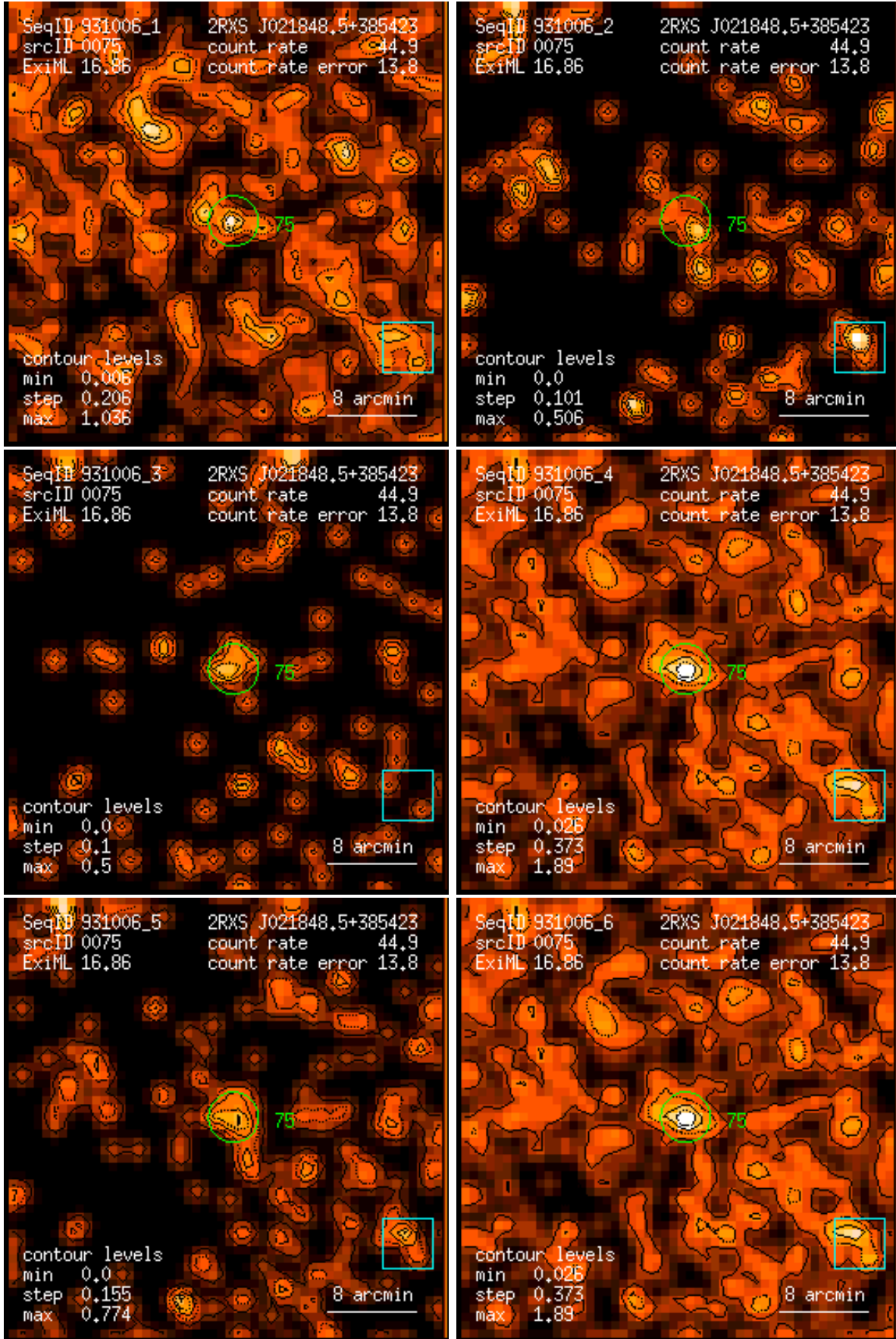
Figure 75: RASS 931006: detection 0075: band rate images, Gaussian filter: (1) PSPC channels 11 – 41, (2) 52 – 90, (3) 91 – 201, (4) 11 – 235, (5) 52 – 201, (6) 11 – 201. Broad band rates in counts/ks. Band rate contour levels in counts/ks/arcmin 2 .
