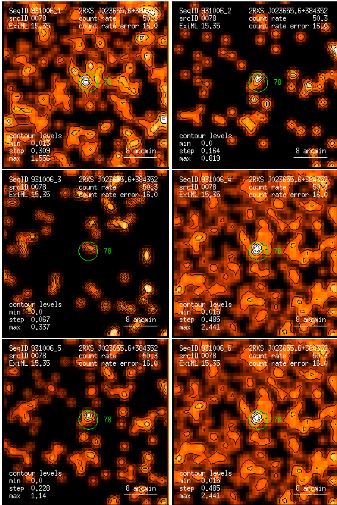
Figure 78: RASS 931006: detection 0078: band rate images, Gaussian filter: (1) PSPC channels 11 – 41, (2) 52 – 90, (3) 91 – 201, (4) 11 – 235, (5) 52 – 201, (6) 11 – 201. Broad band rates in counts/ks. Band rate contour levels in counts/ks/arcmin 2 .
