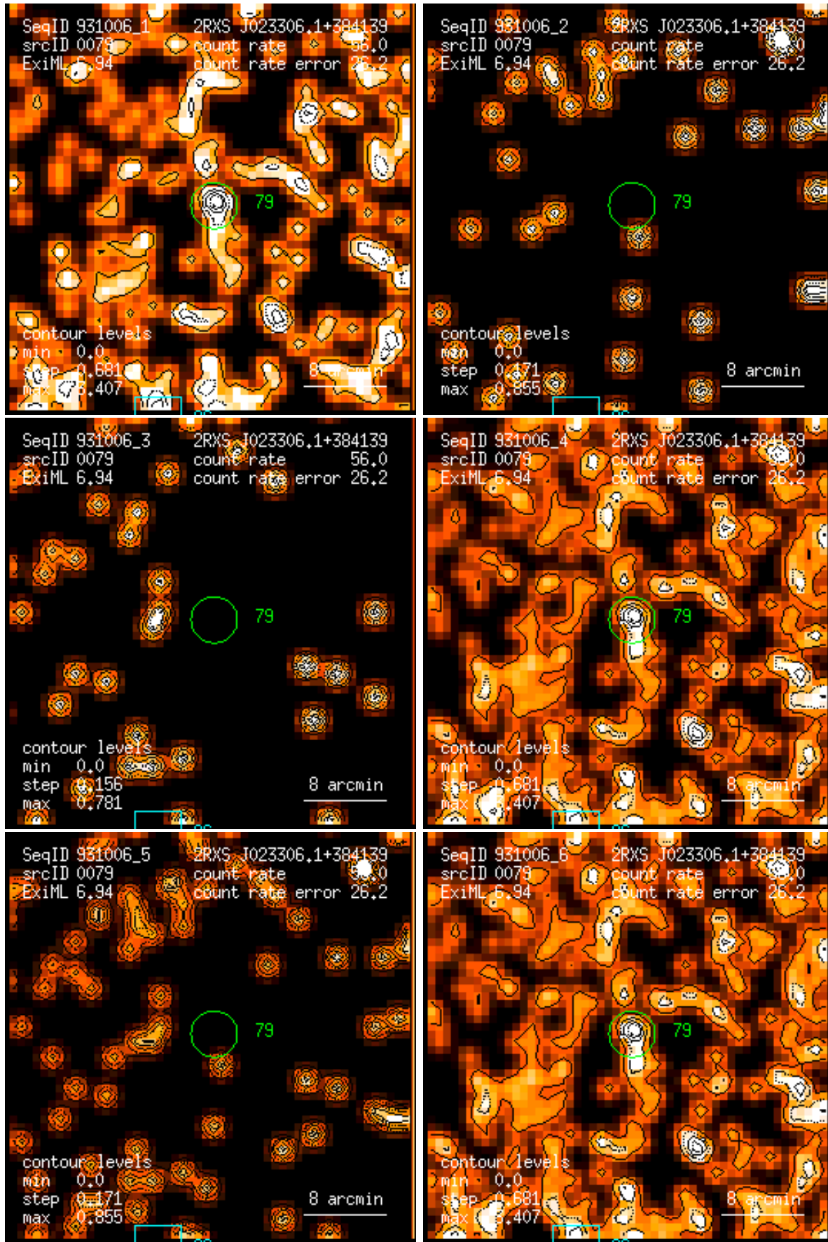
Figure 79: RASS 931006: detection 0079: band rate images, Gaussian filter: (1) PSPC channels 11 – 41, (2) 52 – 90, (3) 91 – 201, (4) 11 – 235, (5) 52 – 201, (6) 11 – 201. Broad band rates in counts/ks. Band rate contour levels in counts/ks/arcmin 2 .
