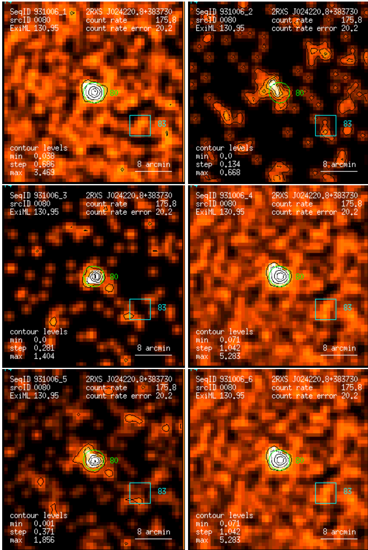
Figure 80: RASS 931006: detection 0080: band rate images, Gaussian filter: (1) PSPC channels 11 – 41, (2) 52 – 90, (3) 91 – 201, (4) 11 – 235, (5) 52 – 201, (6) 11 – 201. Broad band rates in counts/ks. Band rate contour levels in counts/ks/arcmin 2 .
