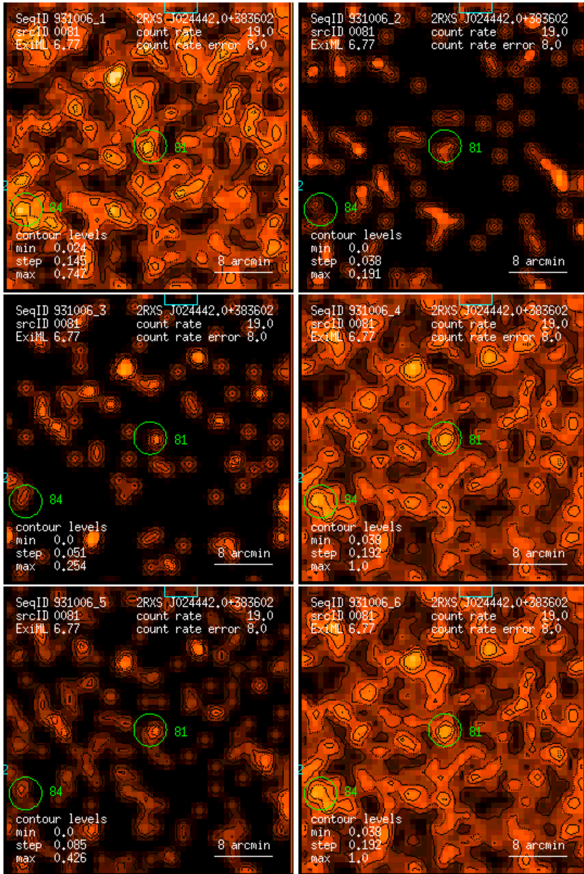
Figure 81: RASS 931006: detection 0081: band rate images, Gaussian filter: (1) PSPC channels 11 – 41, (2) 52 – 90, (3) 91 – 201, (4) 11 – 235, (5) 52 – 201, (6) 11 – 201. Broad band rates in counts/ks. Band rate contour levels in counts/ks/arcmin 2 .
