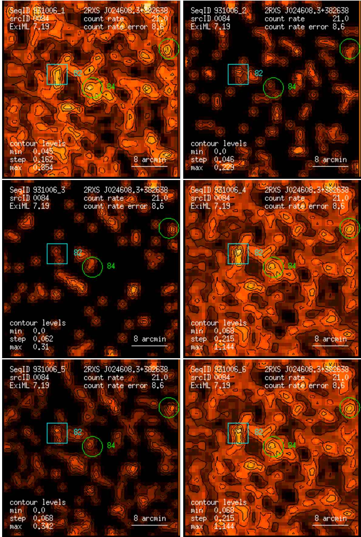
Figure 84: RASS 931006: detection 0084: band rate images, Gaussian filter: (1) PSPC channels 11 – 41, (2) 52 – 90, (3) 91 – 201, (4) 11 – 235, (5) 52 – 201, (6) 11 – 201. Broad band rates in counts/ks. Band rate contour levels in counts/ks/arcmin 2 .
