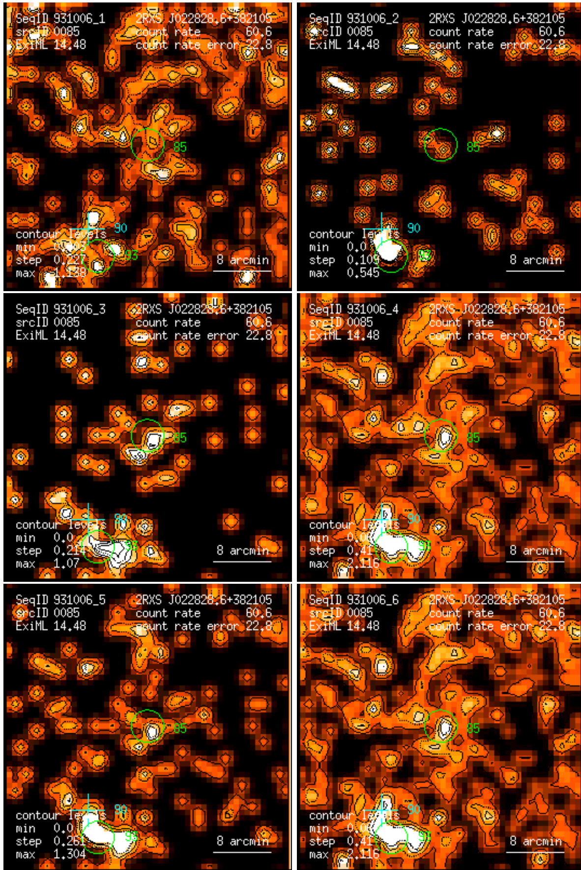
Figure 85: RASS 931006: detection 0085: band rate images, Gaussian filter: (1) PSPC channels 11 – 41, (2) 52 – 90, (3) 91 – 201, (4) 11 – 235, (5) 52 – 201, (6) 11 – 201. Broad band rates in counts/ks. Band rate contour levels in counts/ks/arcmin 2 .
