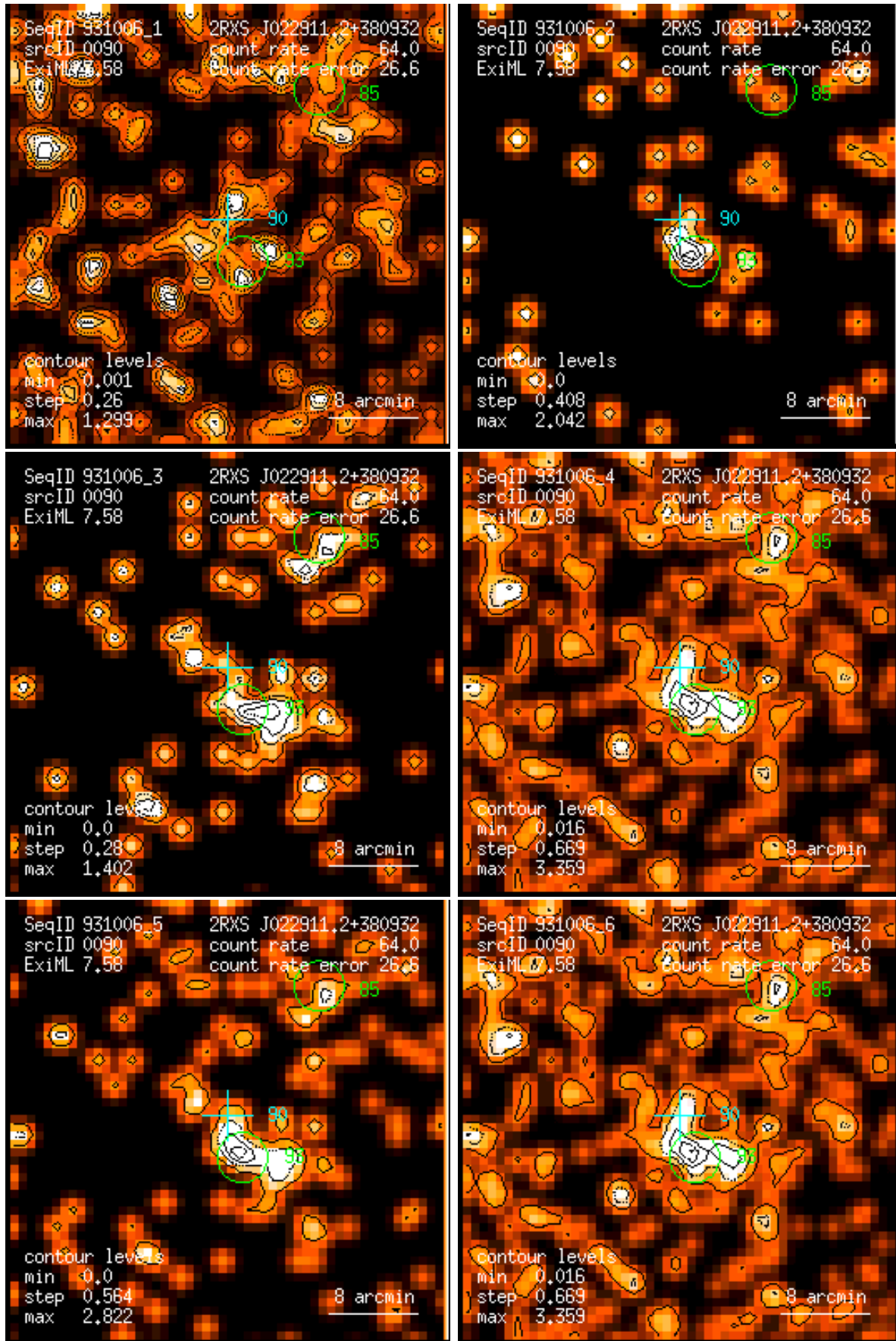
Figure 90: RASS 931006: detection 0090: band rate images, Gaussian filter: (1) PSPC channels 11 – 41, (2) 52 – 90, (3) 91 – 201, (4) 11 – 235, (5) 52 – 201, (6) 11 – 201. Broad band rates in counts/ks. Band rate contour levels in counts/ks/arcmin 2 .
