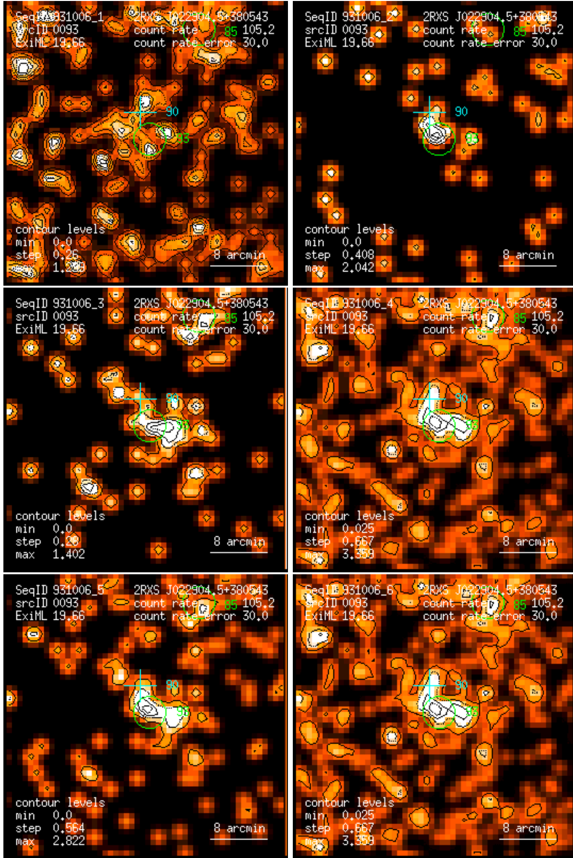
Figure 93: RASS 931006: detection 0093: band rate images, Gaussian filter: (1) PSPC channels 11 – 41, (2) 52 – 90, (3) 91 – 201, (4) 11 – 235, (5) 52 – 201, (6) 11 – 201. Broad band rates in counts/ks. Band rate contour levels in counts/ks/arcmin 2 .
