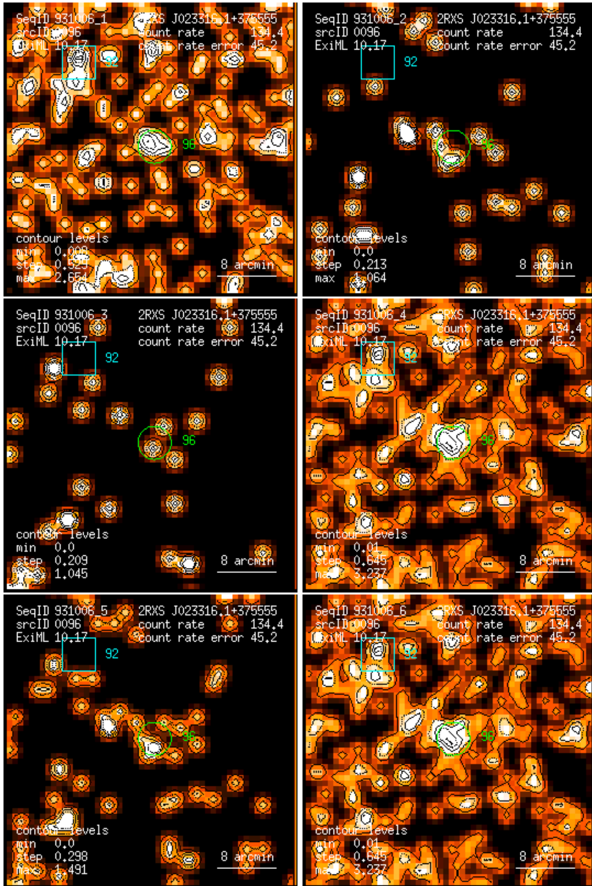
Figure 96: RASS 931006: detection 0096: band rate images, Gaussian filter: (1) PSPC channels 11 – 41, (2) 52 – 90, (3) 91 – 201, (4) 11 – 235, (5) 52 – 201, (6) 11 – 201. Broad band rates in counts/ks. Band rate contour levels in counts/ks/arcmin 2 .
