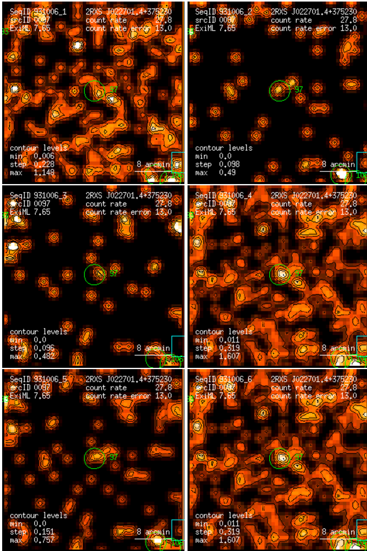
Figure 97: RASS 931006: detection 0097: band rate images, Gaussian filter: (1) PSPC channels 11 – 41, (2) 52 – 90, (3) 91 – 201, (4) 11 – 235, (5) 52 – 201, (6) 11 – 201. Broad band rates in counts/ks. Band rate contour levels in counts/ks/arcmin 2 .
