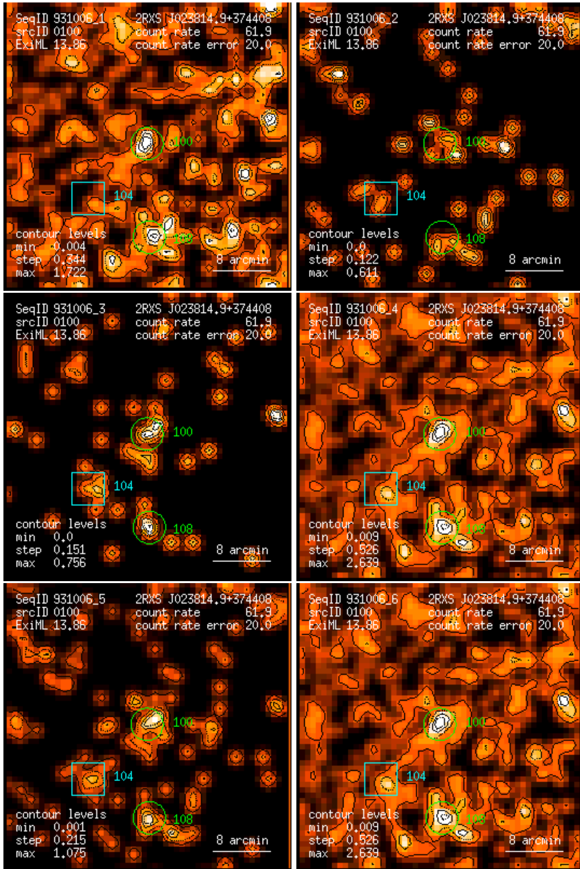
Figure 100: RASS 931006: detection 0100: band rate images, Gaussian filter: (1) PSPC channels 11 – 41, (2) 52 – 90, (3) 91 – 201, (4) 11 – 235, (5) 52 – 201, (6) 11 – 201. Broad band rates in counts/ks. Band rate contour levels in counts/ks/arcmin 2 .
