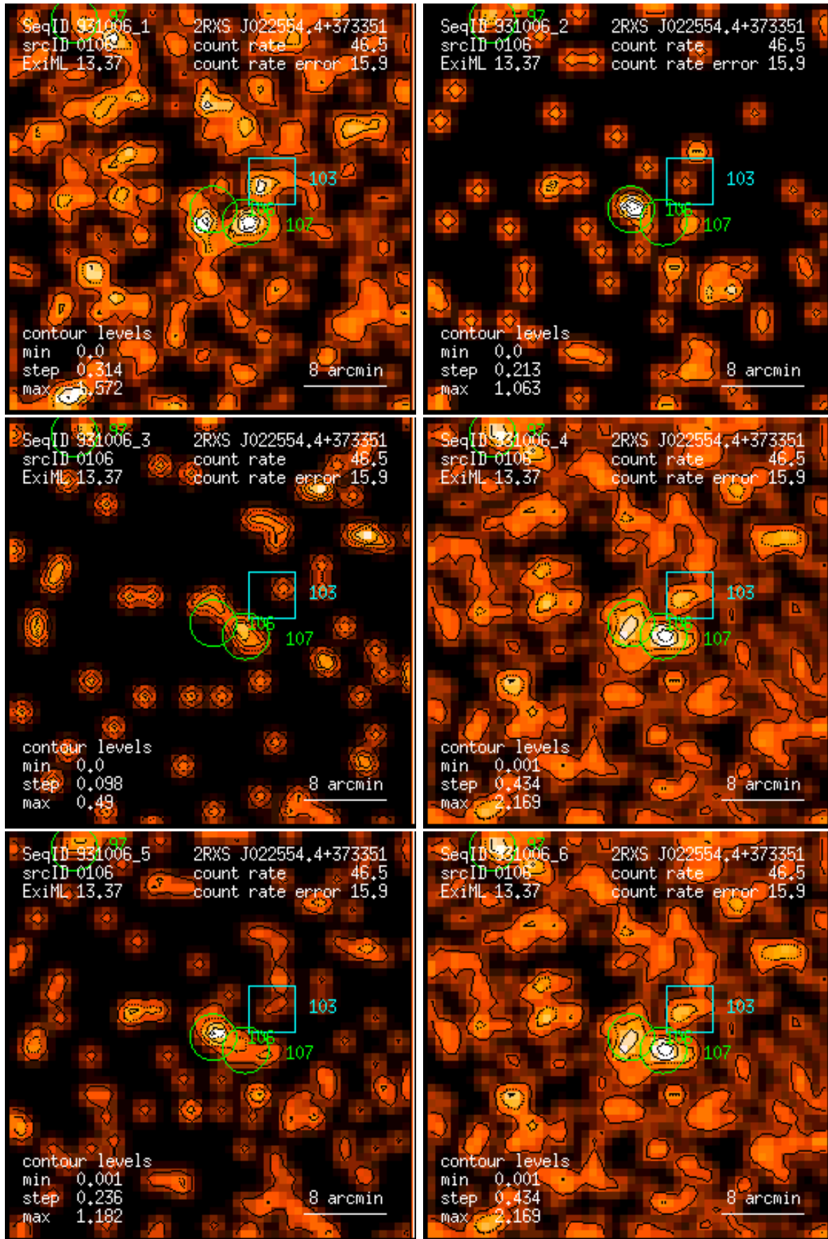
Figure 106: RASS 931006: detection 0106: band rate images, Gaussian filter: (1) PSPC channels 11 – 41, (2) 52 – 90, (3) 91 – 201, (4) 11 – 235, (5) 52 – 201, (6) 11 – 201. Broad band rates in counts/ks. Band rate contour levels in counts/ks/arcmin 2 .
