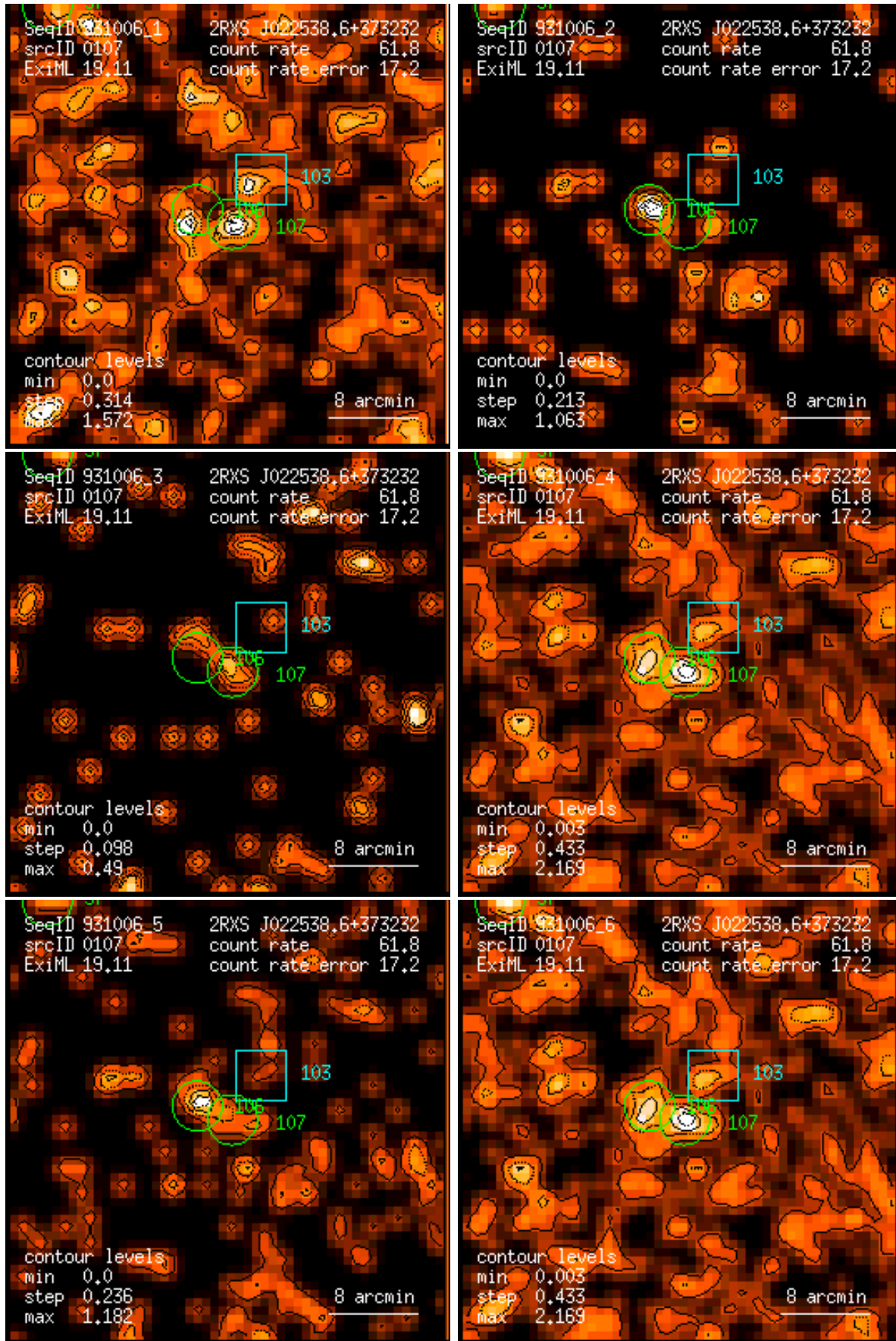
Figure 107: RASS 931006: detection 0107: band rate images, Gaussian filter: (1) PSPC channels 11 – 41, (2) 52 – 90, (3) 91 – 201, (4) 11 – 235, (5) 52 – 201, (6) 11 – 201. Broad band rates in counts/ks. Band rate contour levels in counts/ks/arcmin 2 .
