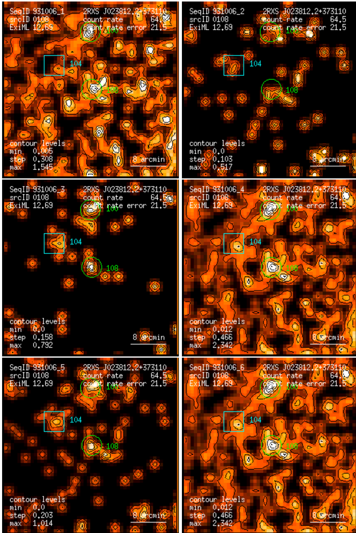
Figure 108: RASS 931006: detection 0108: band rate images, Gaussian filter: (1) PSPC channels 11 – 41, (2) 52 – 90, (3) 91 – 201, (4) 11 – 235, (5) 52 – 201, (6) 11 – 201. Broad band rates in counts/ks. Band rate contour levels in counts/ks/arcmin 2 .
