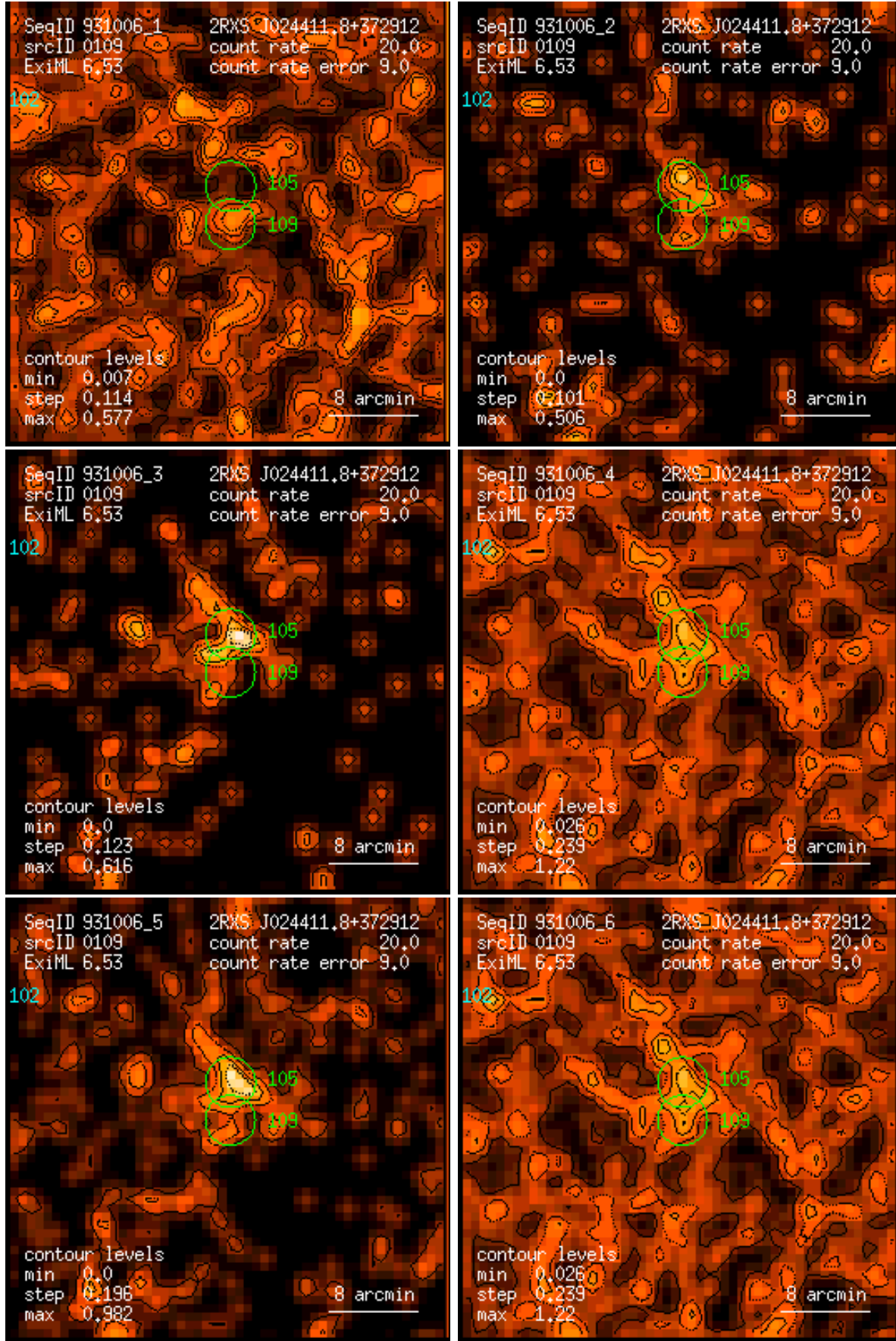
Figure 109: RASS 931006: detection 0109: band rate images, Gaussian filter: (1) PSPC channels 11 – 41, (2) 52 – 90, (3) 91 – 201, (4) 11 – 235, (5) 52 – 201, (6) 11 – 201. Broad band rates in counts/ks. Band rate contour levels in counts/ks/arcmin 2 .
