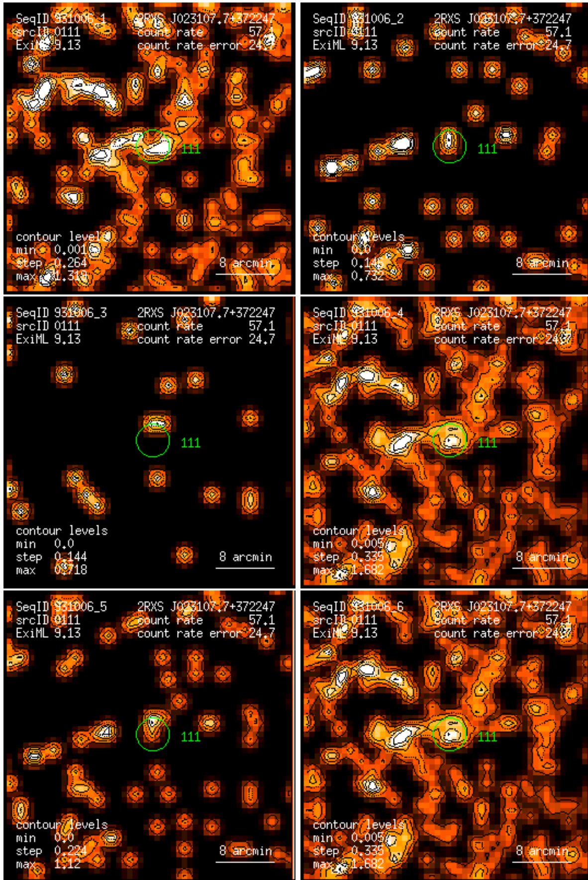
Figure 111: RASS 931006: detection 0111: band rate images, Gaussian filter: (1) PSPC channels 11 – 41, (2) 52 – 90, (3) 91 – 201, (4) 11 – 235, (5) 52 – 201, (6) 11 – 201. Broad band rates in counts/ks. Band rate contour levels in counts/ks/arcmin 2 .
