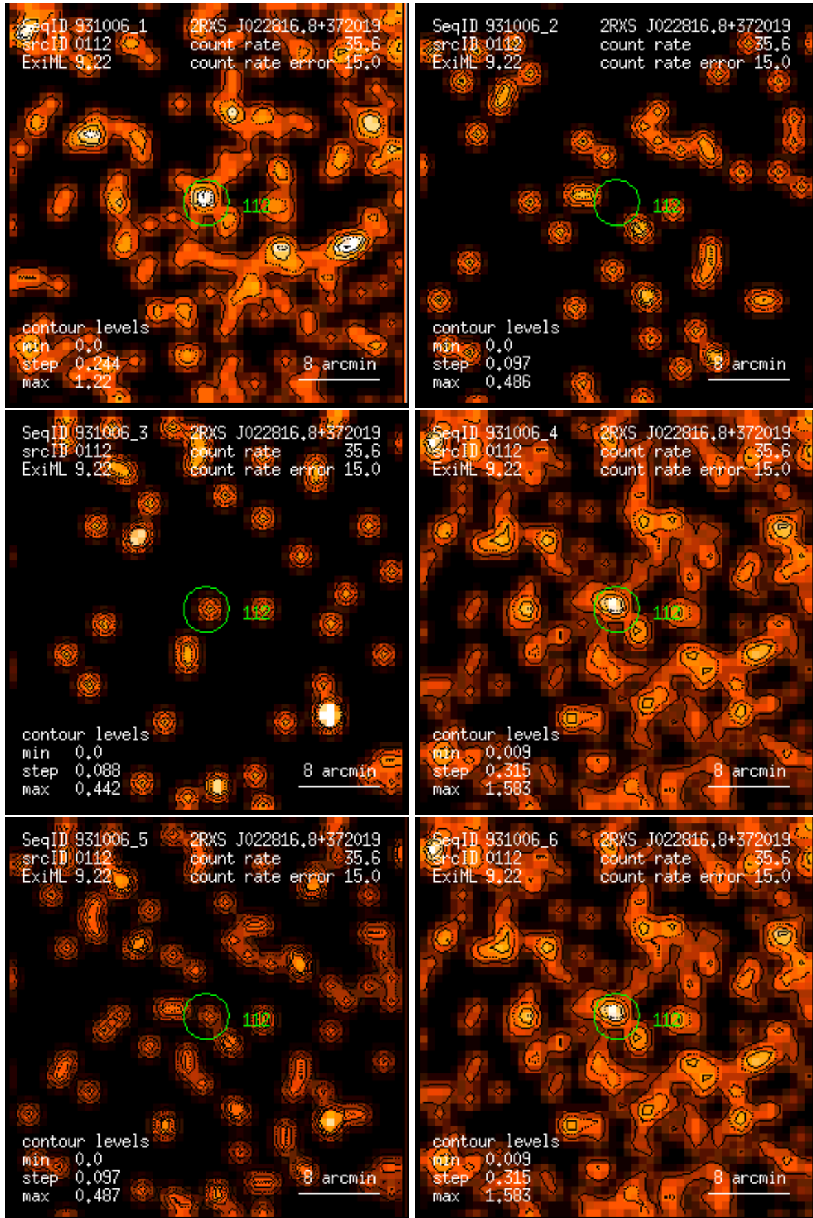
Figure 112: RASS 931006: detection 0112: band rate images, Gaussian filter: (1) PSPC channels 11 – 41, (2) 52 – 90, (3) 91 – 201, (4) 11 – 235, (5) 52 – 201, (6) 11 – 201. Broad band rates in counts/ks. Band rate contour levels in counts/ks/arcmin 2 .
