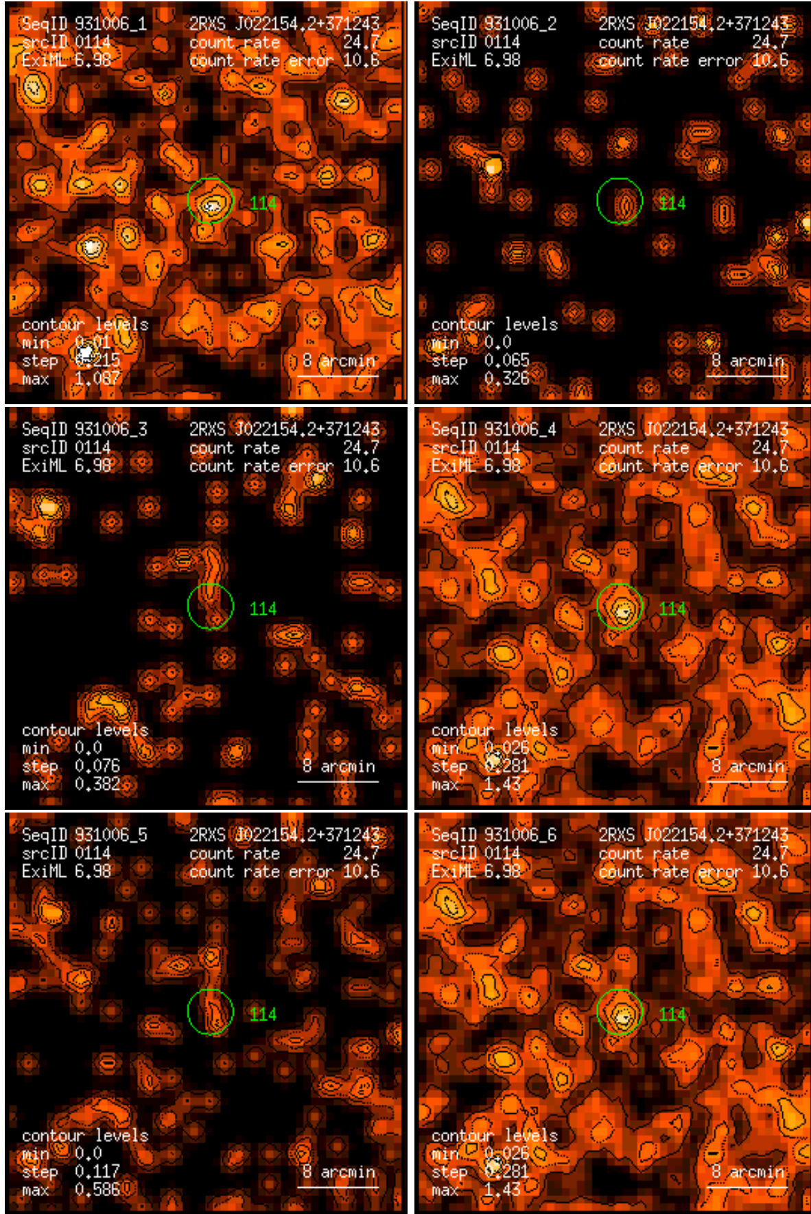
Figure 114: RASS 931006: detection 0114: band rate images, Gaussian filter: (1) PSPC channels 11 – 41, (2) 52 – 90, (3) 91 – 201, (4) 11 – 235, (5) 52 – 201, (6) 11 – 201. Broad band rates in counts/ks. Band rate contour levels in counts/ks/arcmin 2 .
