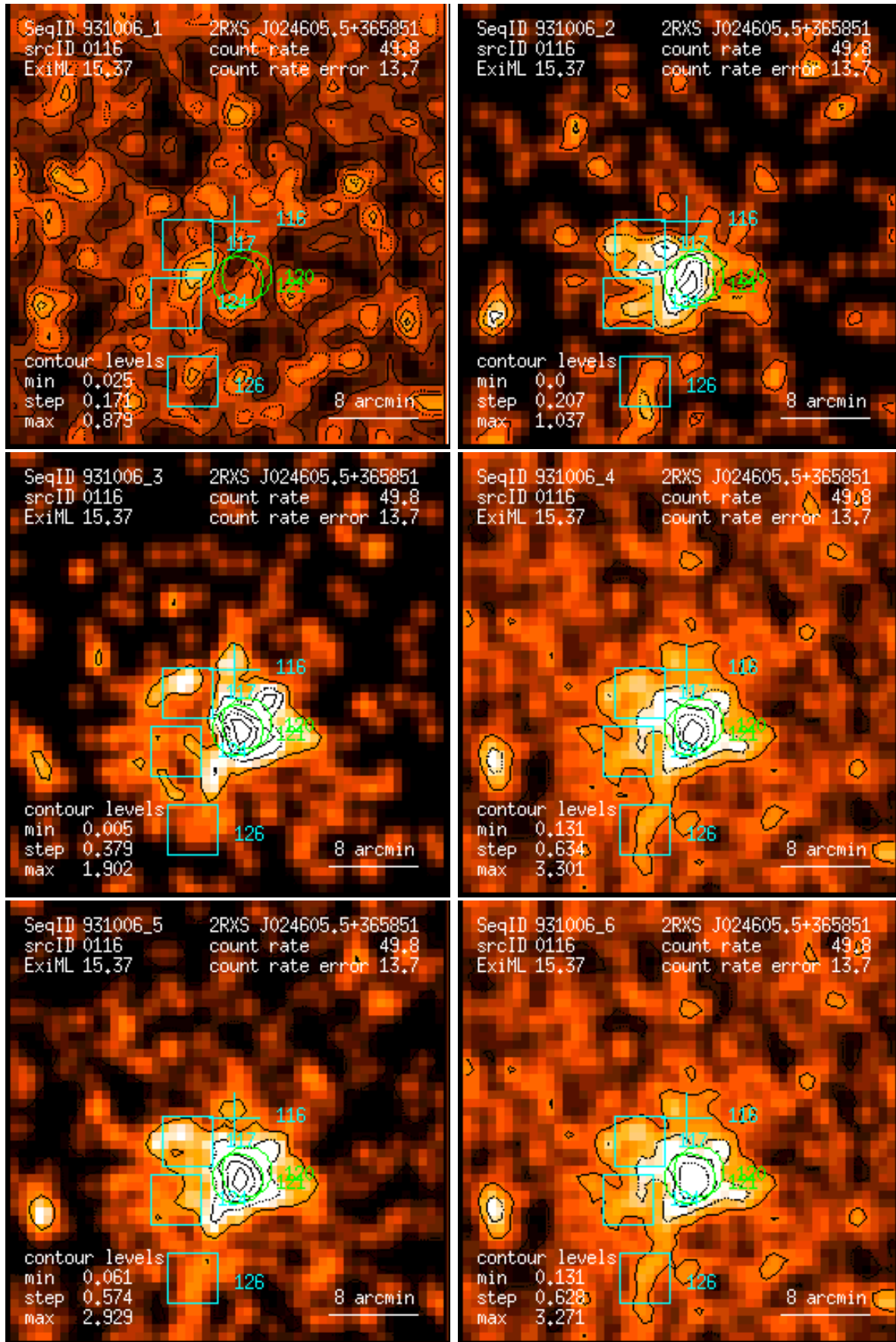
Figure 116: RASS 931006: detection 0116: band rate images, Gaussian filter: (1) PSPC channels 11 – 41, (2) 52 – 90, (3) 91 – 201, (4) 11 – 235, (5) 52 – 201, (6) 11 – 201. Broad band rates in counts/ks. Band rate contour levels in counts/ks/arcmin 2 .
