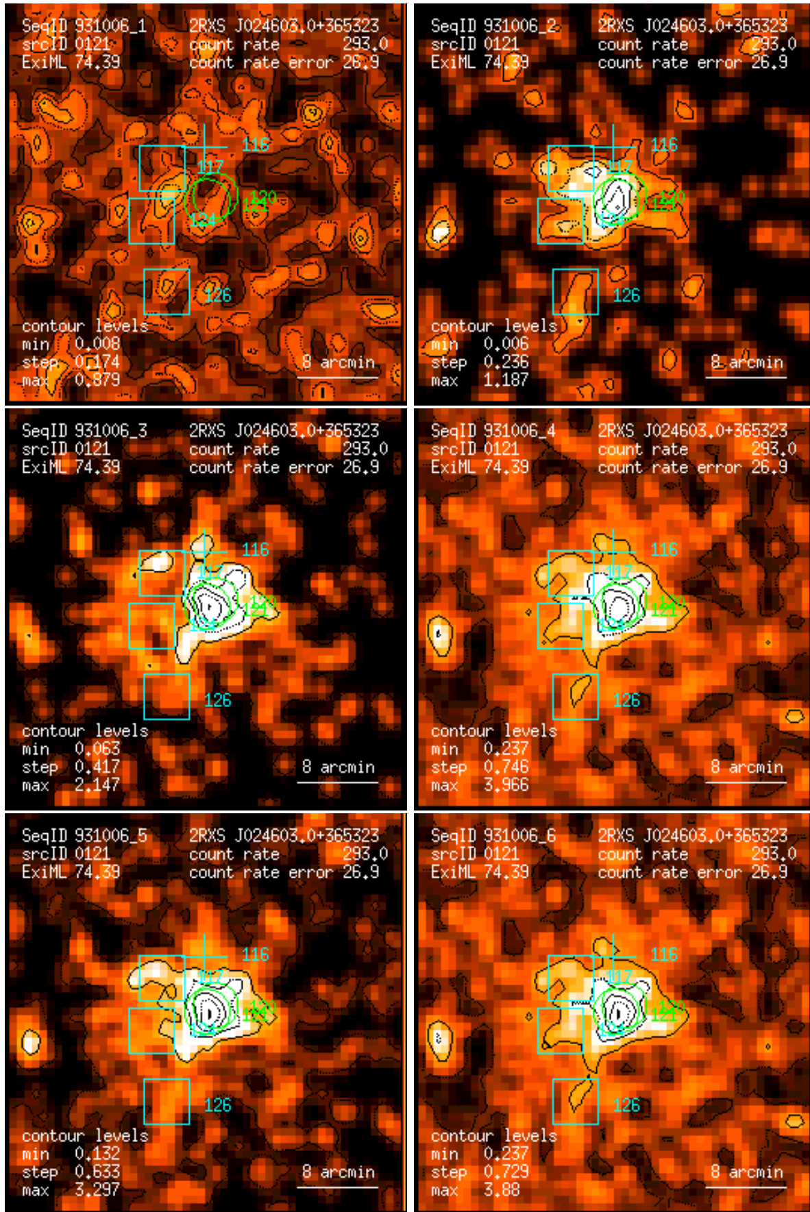
Figure 121: RASS 931006: detection 0121: band rate images, Gaussian filter: (1) PSPC channels 11 – 41, (2) 52 – 90, (3) 91 – 201, (4) 11 – 235, (5) 52 – 201, (6) 11 – 201. Broad band rates in counts/ks. Band rate contour levels in counts/ks/arcmin 2 .
