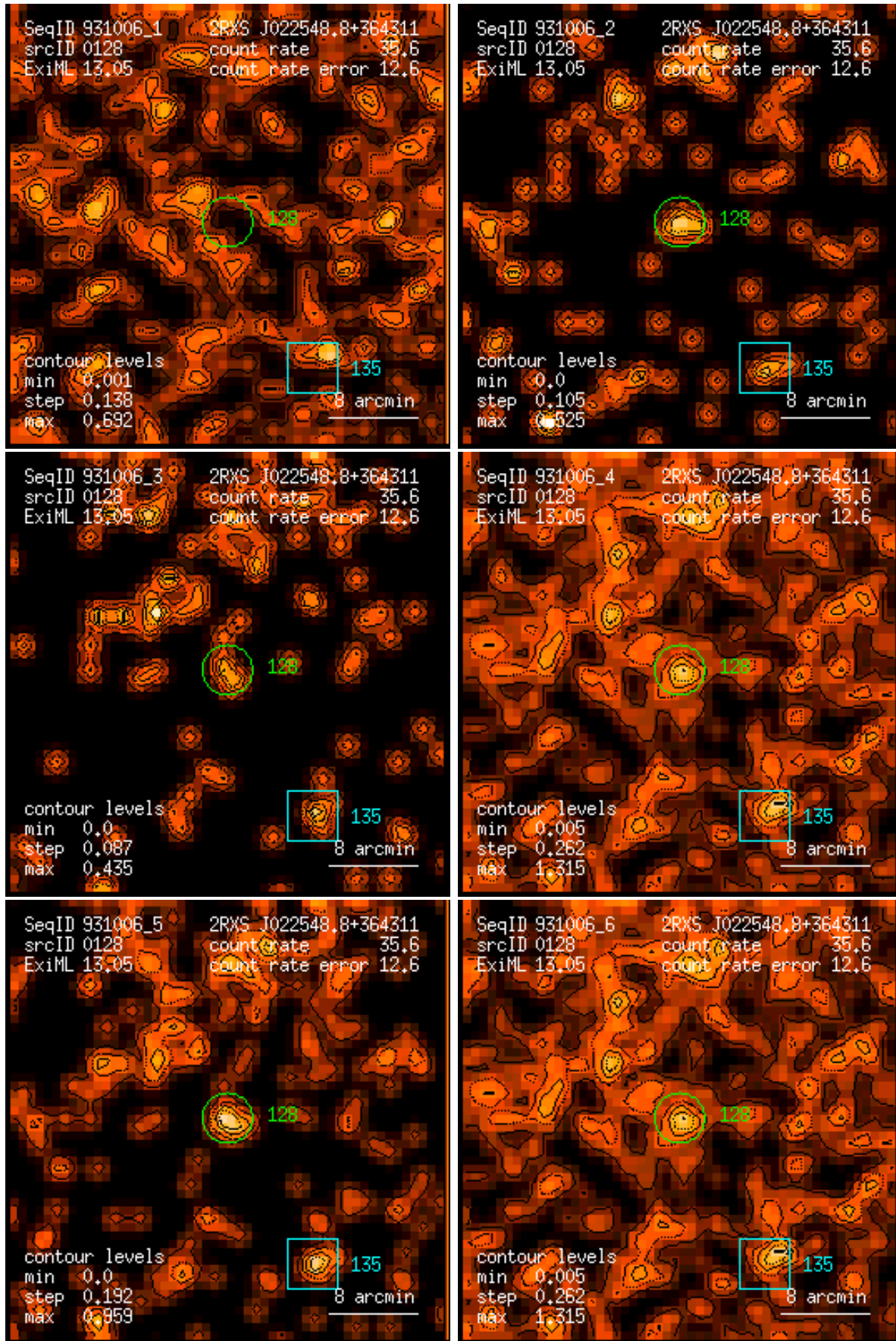
Figure 128: RASS 931006: detection 0128: band rate images, Gaussian filter: (1) PSPC channels 11 – 41, (2) 52 – 90, (3) 91 – 201, (4) 11 – 235, (5) 52 – 201, (6) 11 – 201. Broad band rates in counts/ks. Band rate contour levels in counts/ks/arcmin 2 .
