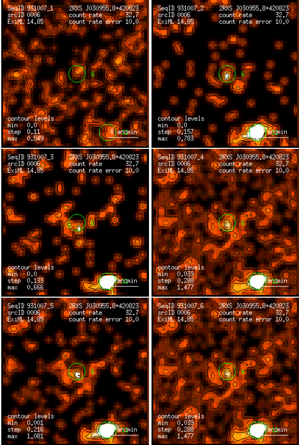
Figure 6: RASS 931007: detection 0006: band rate images, Gaussian filter: (1) PSPC channels 11 – 41, (2) 52 – 90, (3) 91 – 201, (4) 11 – 235, (5) 52 – 201, (6) 11 – 201. Broad band rates in counts/ks. Band rate contour levels in counts/ks/arcmin 2 .
