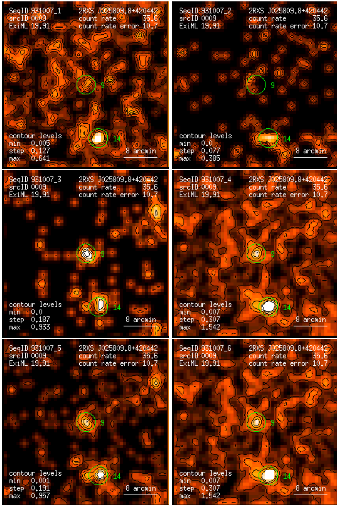
Figure 9: RASS 931007: detection 0009: band rate images, Gaussian filter: (1) PSPC channels 11 – 41, (2) 52 – 90, (3) 91 – 201, (4) 11 – 235, (5) 52 – 201, (6) 11 – 201. Broad band rates in counts/ks. Band rate contour levels in counts/ks/arcmin 2 .
