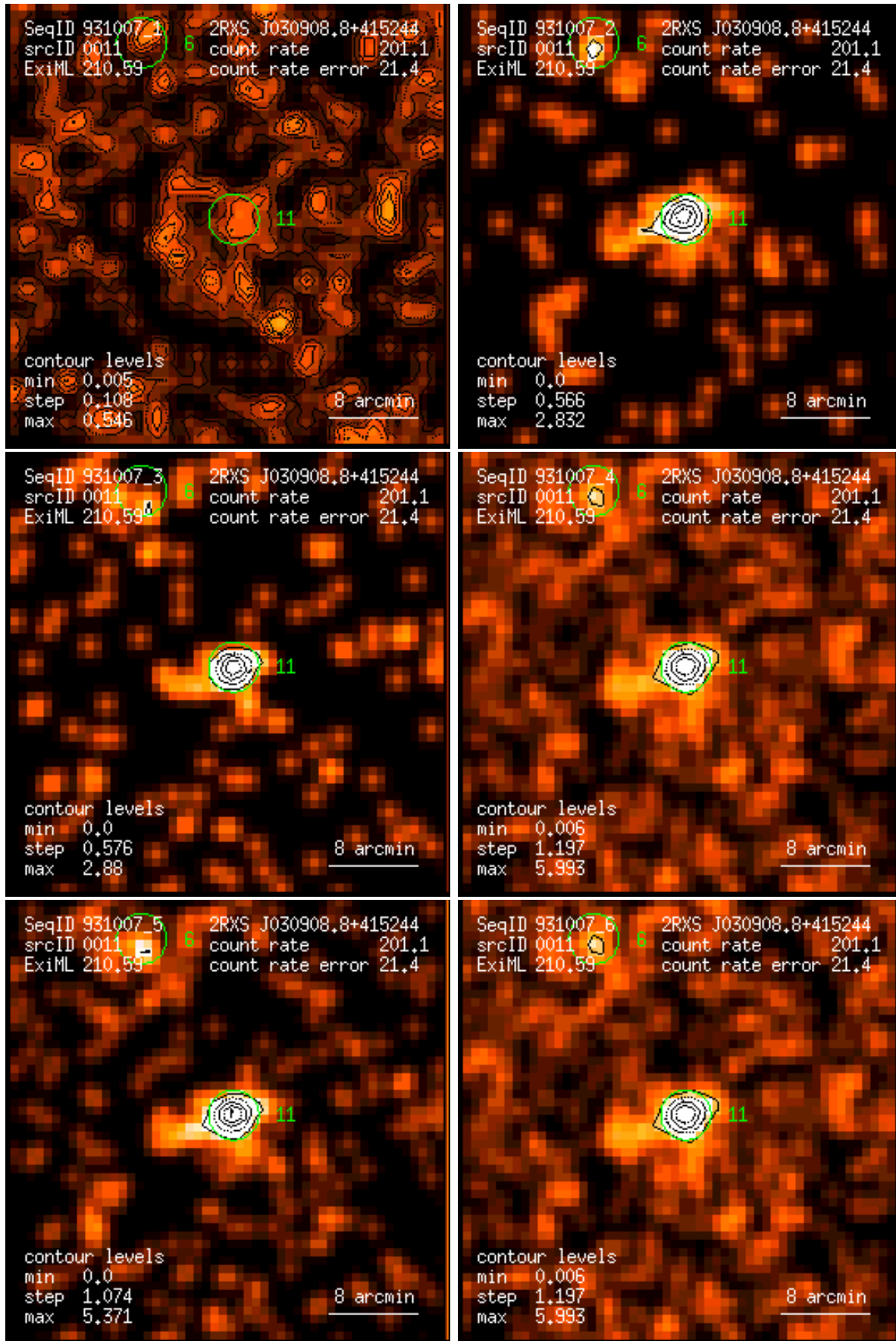
Figure 11: RASS 931007: detection 0011: band rate images, Gaussian filter: (1) PSPC channels 11 – 41, (2) 52 – 90, (3) 91 – 201, (4) 11 – 235, (5) 52 – 201, (6) 11 – 201. Broad band rates in counts/ks. Band rate contour levels in counts/ks/arcmin 2 .
