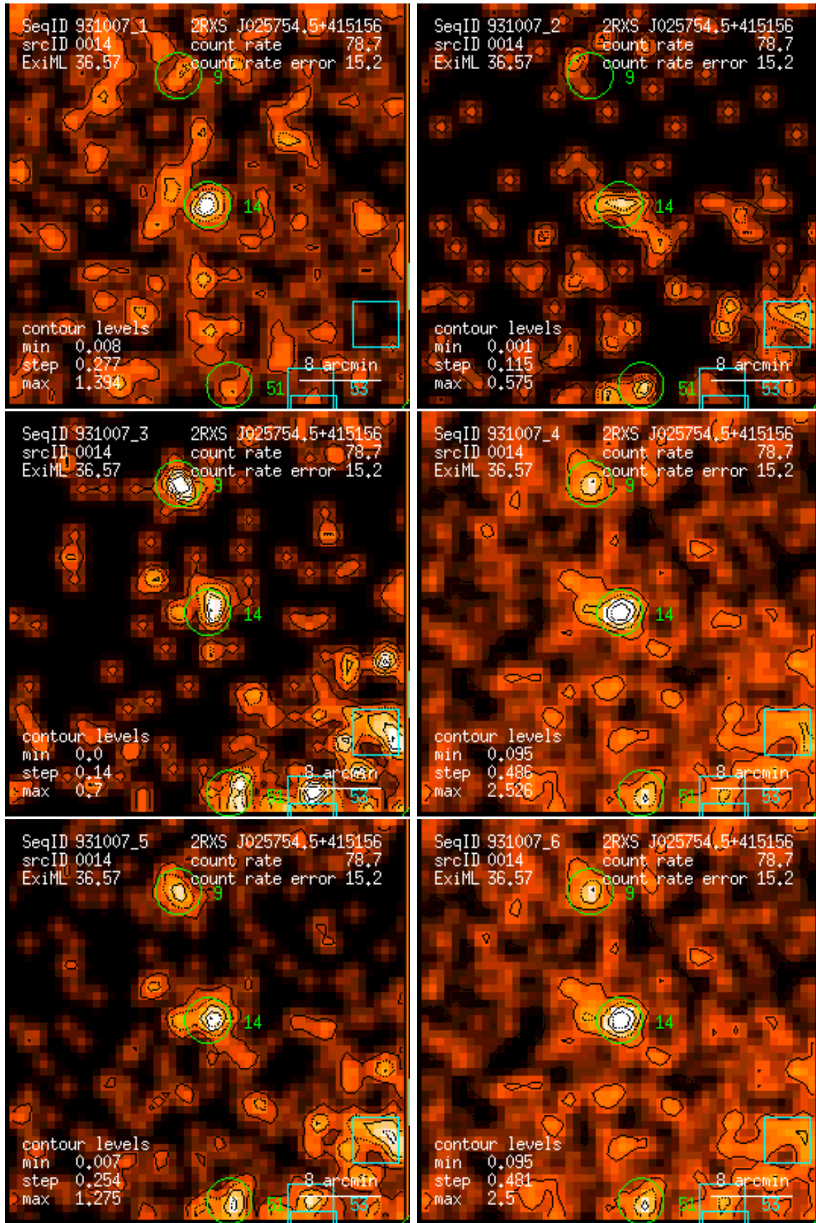
Figure 14: RASS 931007: detection 0014: band rate images, Gaussian filter: (1) PSPC channels 11 – 41, (2) 52 – 90, (3) 91 – 201, (4) 11 – 235, (5) 52 – 201, (6) 11 – 201. Broad band rates in counts/ks. Band rate contour levels in counts/ks/arcmin 2 .
