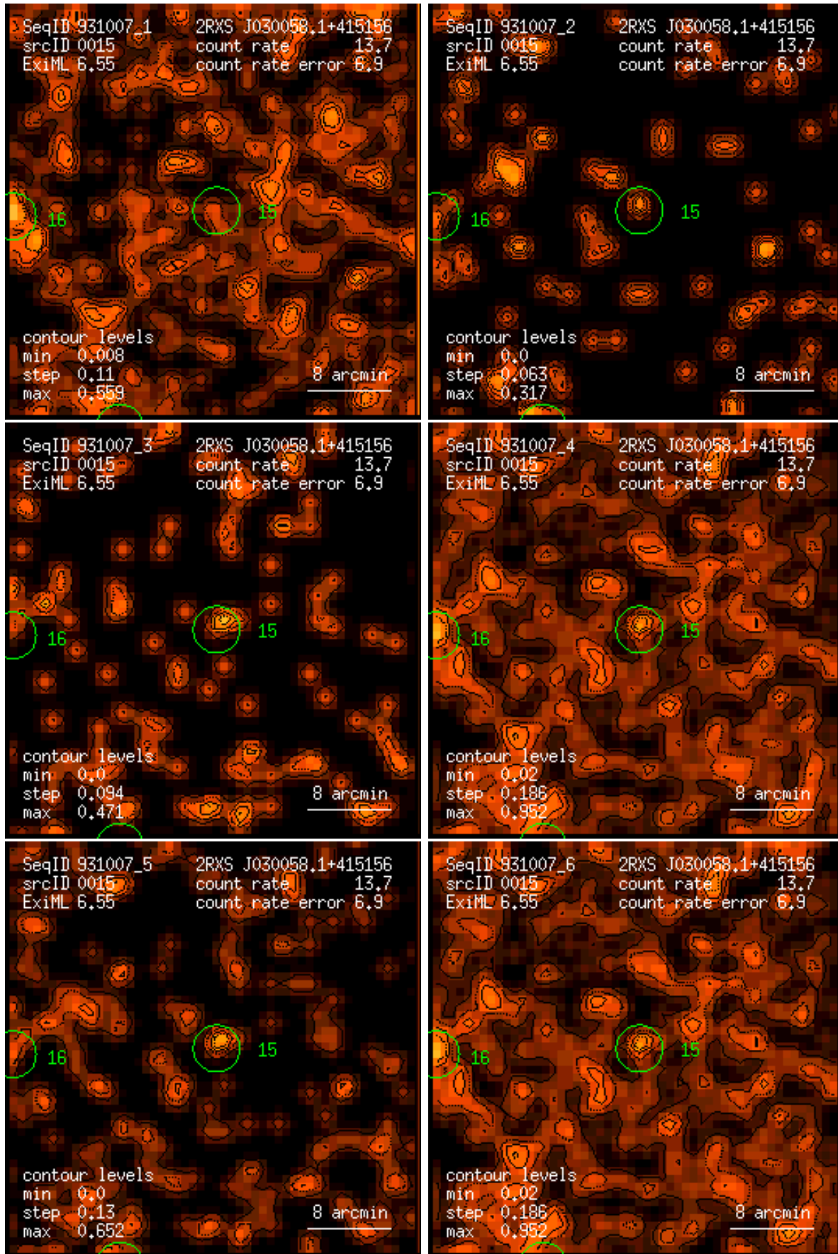
Figure 15: RASS 931007: detection 0015: band rate images, Gaussian filter: (1) PSPC channels 11 – 41, (2) 52 – 90, (3) 91 – 201, (4) 11 – 235, (5) 52 – 201, (6) 11 – 201. Broad band rates in counts/ks. Band rate contour levels in counts/ks/arcmin 2 .
