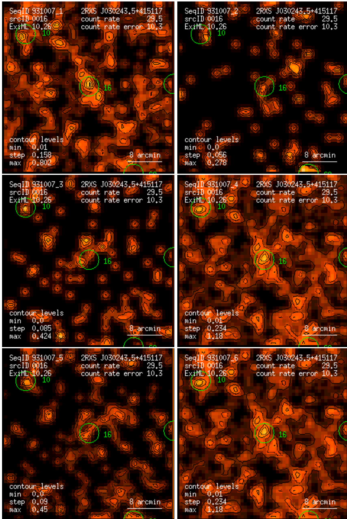
Figure 16: RASS 931007: detection 0016: band rate images, Gaussian filter: (1) PSPC channels 11 – 41, (2) 52 – 90, (3) 91 – 201, (4) 11 – 235, (5) 52 – 201, (6) 11 – 201. Broad band rates in counts/ks. Band rate contour levels in counts/ks/arcmin 2 .
