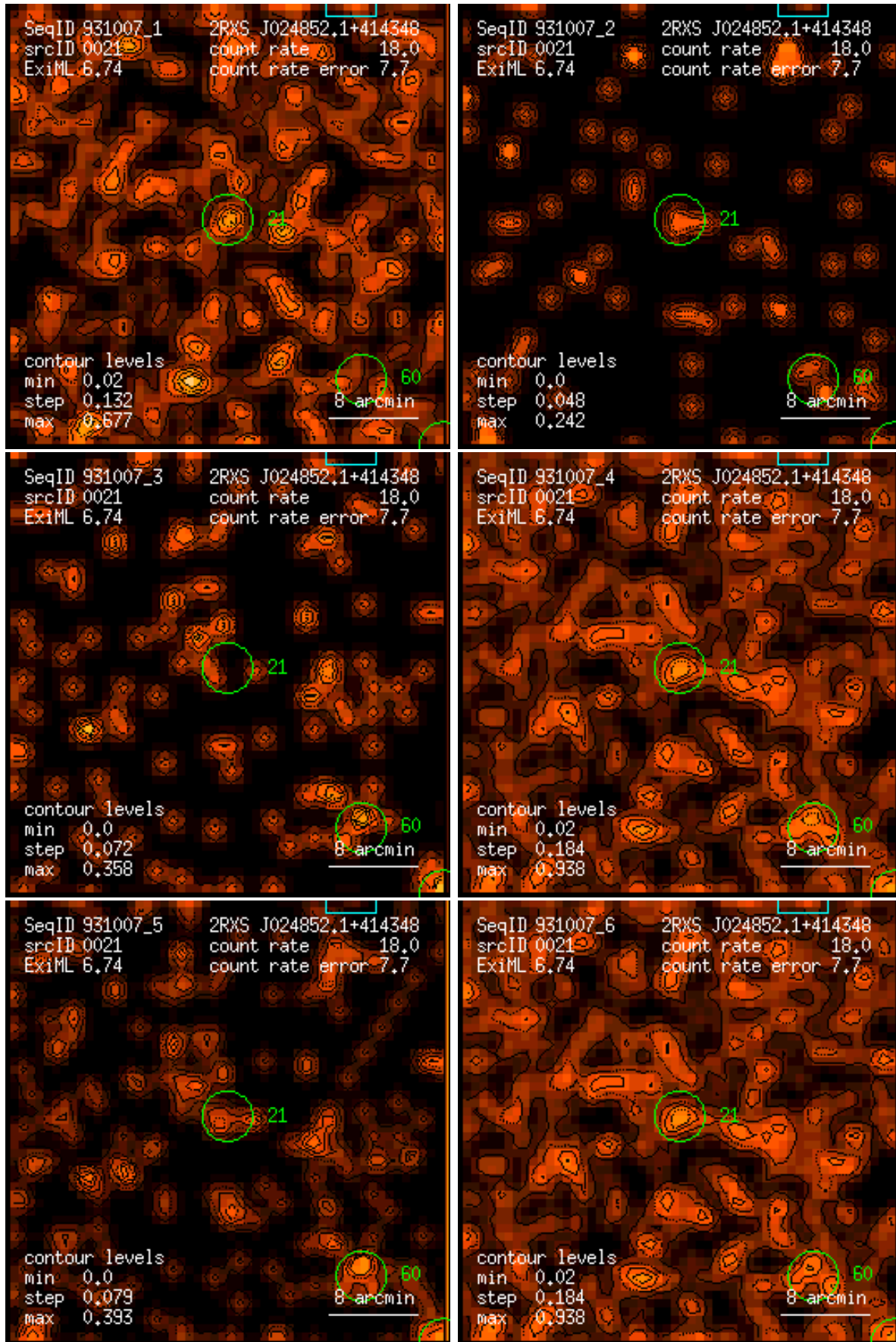
Figure 21: RASS 931007: detection 0021: band rate images, Gaussian filter: (1) PSPC channels 11 – 41, (2) 52 – 90, (3) 91 – 201, (4) 11 – 235, (5) 52 – 201, (6) 11 – 201. Broad band rates in counts/ks. Band rate contour levels in counts/ks/arcmin 2 .
