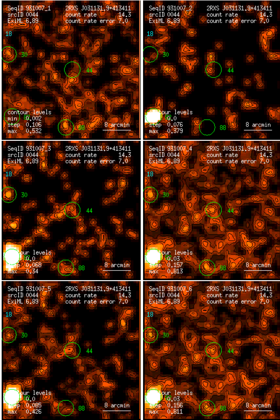
Figure 44: RASS 931007: detection 0044: band rate images, Gaussian filter: (1) PSPC channels 11 – 41, (2) 52 – 90, (3) 91 – 201, (4) 11 – 235, (5) 52 – 201, (6) 11 – 201. Broad band rates in counts/ks. Band rate contour levels in counts/ks/arcmin 2 .
