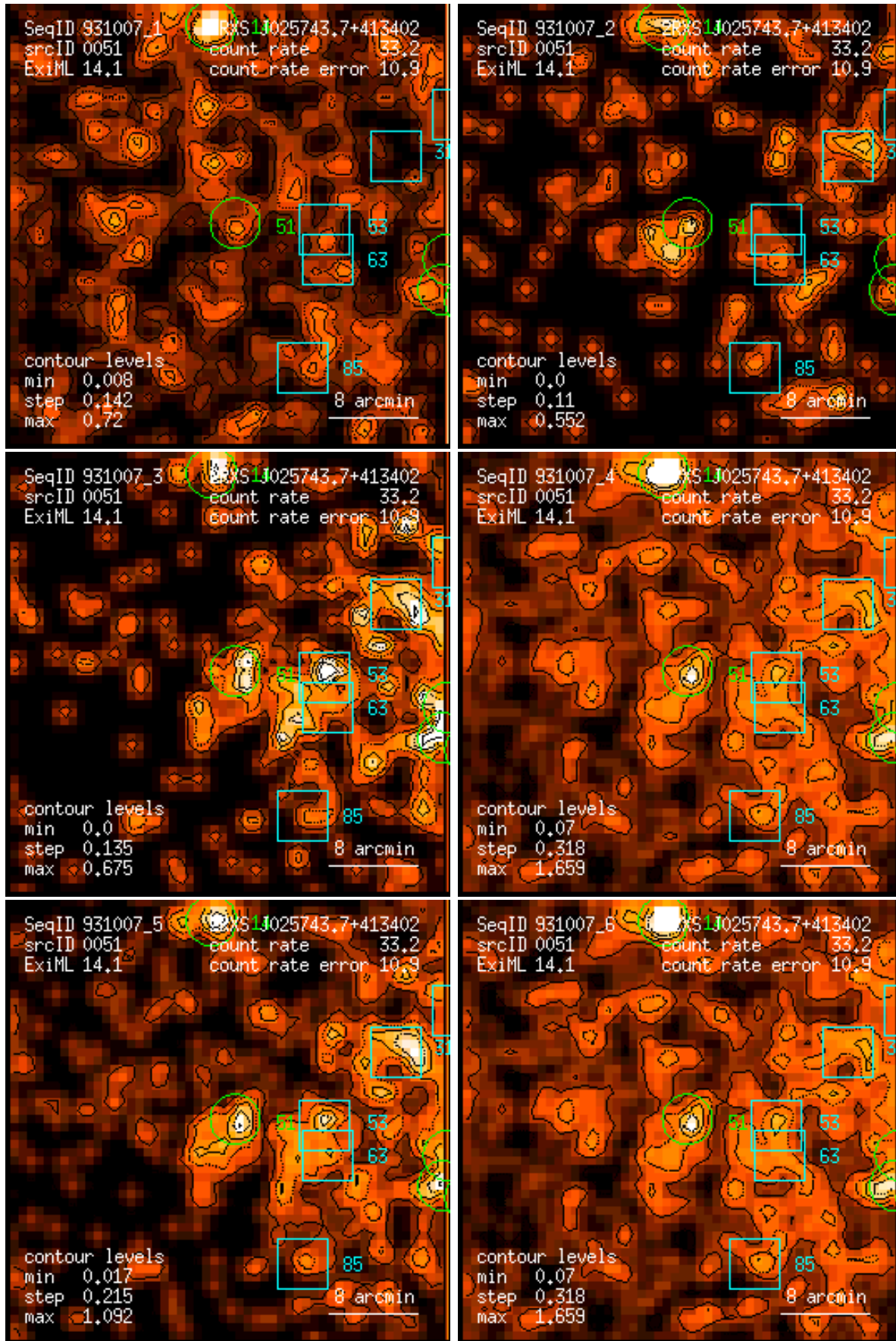
Figure 51: RASS 931007: detection 0051: band rate images, Gaussian filter: (1) PSPC channels 11 – 41, (2) 52 – 90, (3) 91 – 201, (4) 11 – 235, (5) 52 – 201, (6) 11 – 201. Broad band rates in counts/ks. Band rate contour levels in counts/ks/arcmin 2 .
