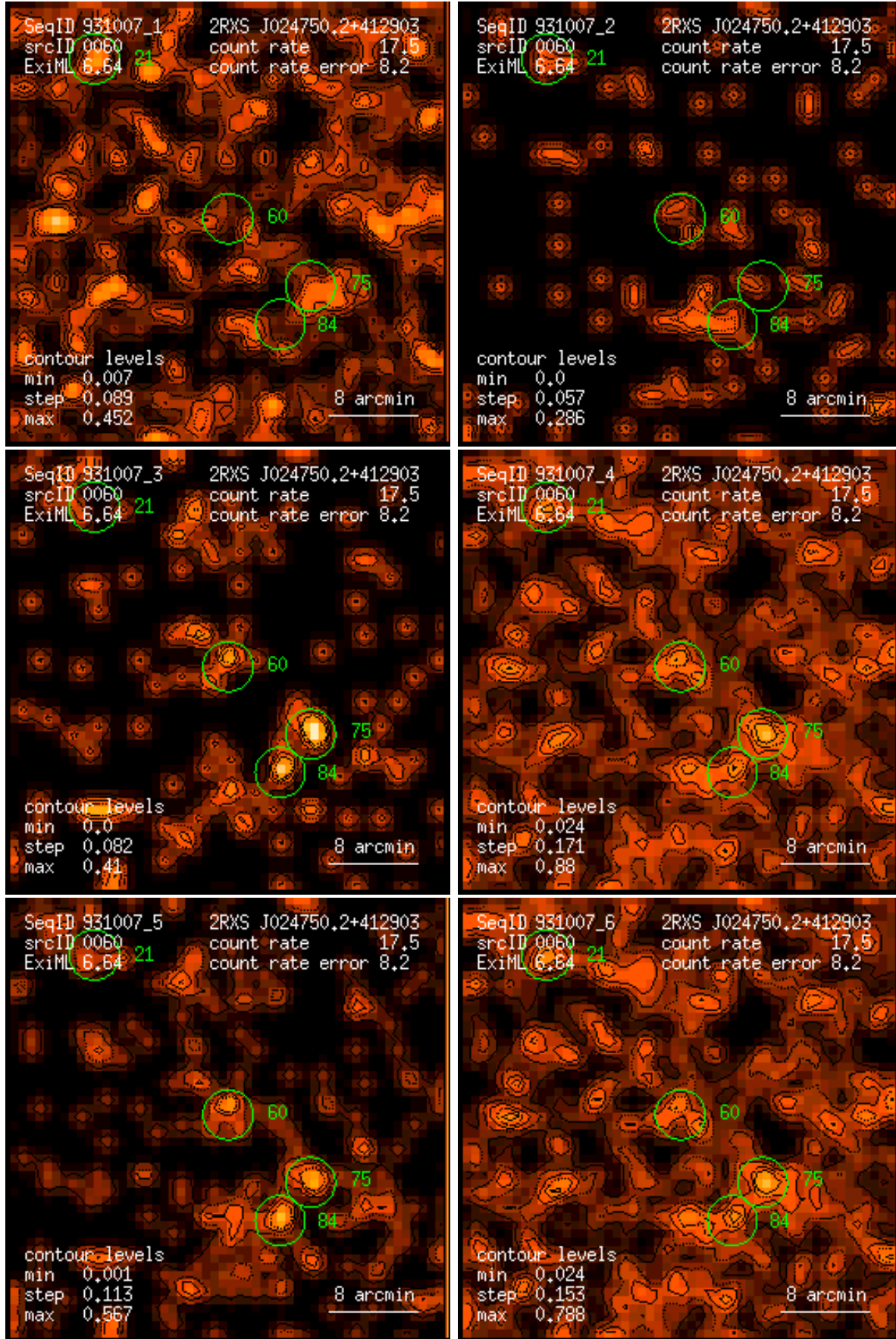
Figure 60: RASS 931007: detection 0060: band rate images, Gaussian filter: (1) PSPC channels 11 – 41, (2) 52 – 90, (3) 91 – 201, (4) 11 – 235, (5) 52 – 201, (6) 11 – 201. Broad band rates in counts/ks. Band rate contour levels in counts/ks/arcmin 2 .
