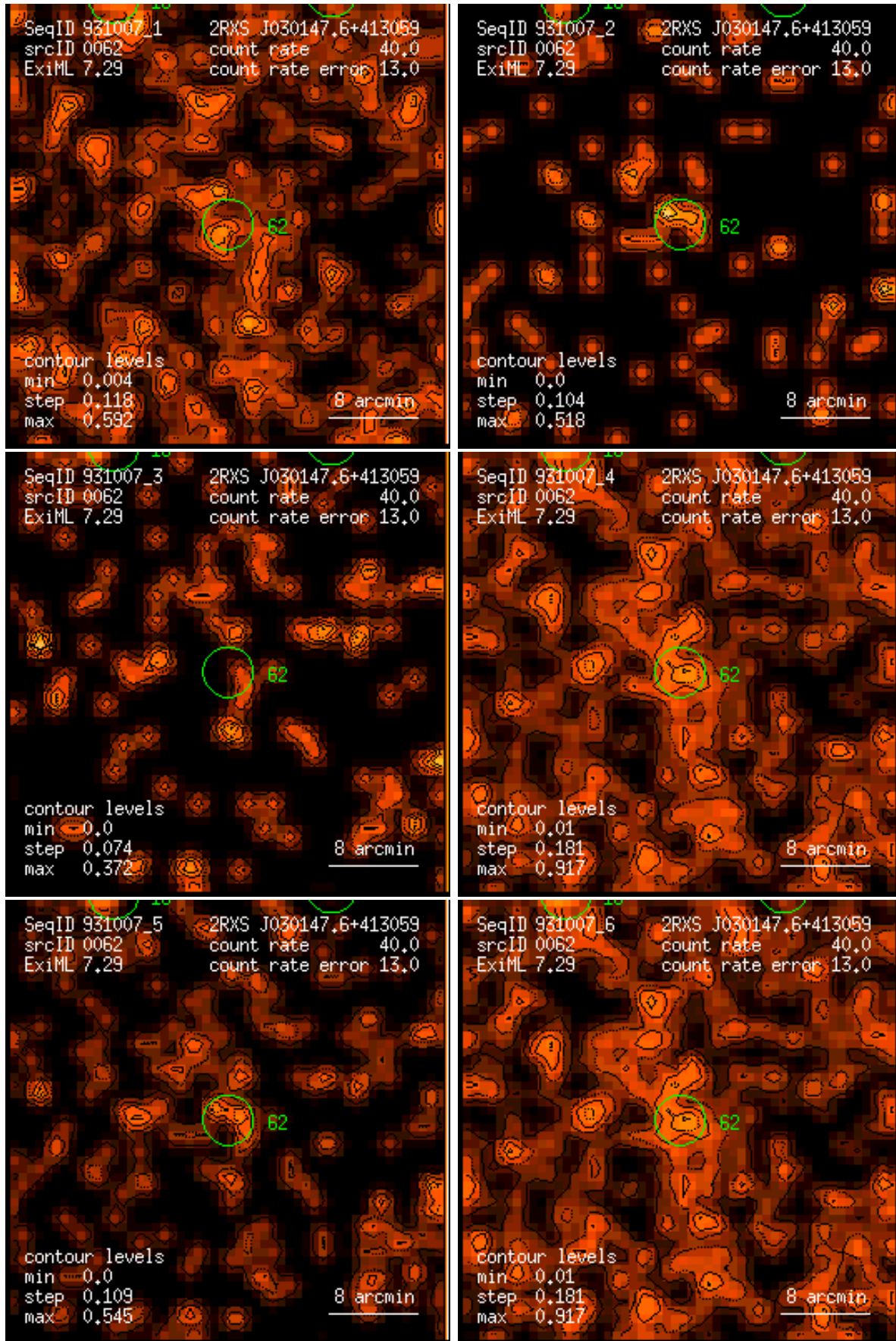
Figure 62: RASS 931007: detection 0062: band rate images, Gaussian filter: (1) PSPC channels 11 – 41, (2) 52 – 90, (3) 91 – 201, (4) 11 – 235, (5) 52 – 201, (6) 11 – 201. Broad band rates in counts/ks. Band rate contour levels in counts/ks/arcmin 2 .
