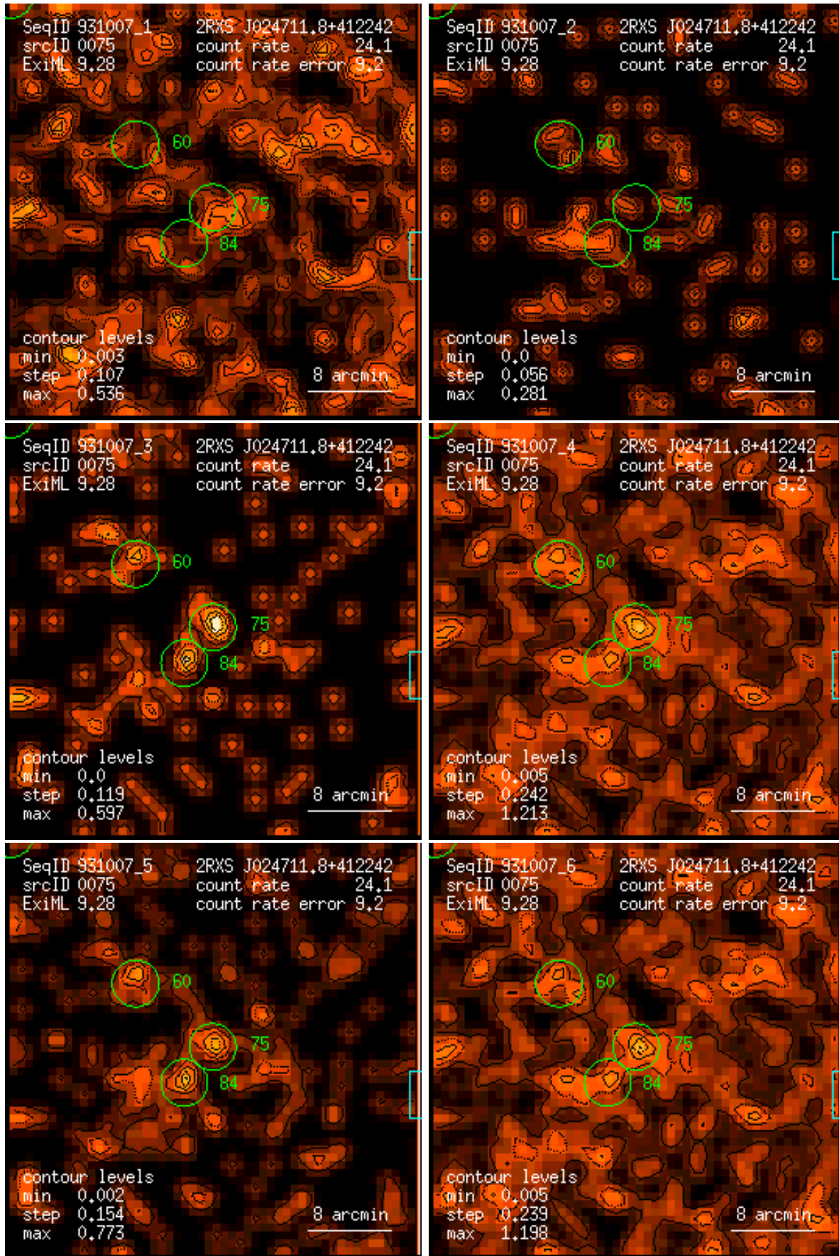
Figure 75: RASS 931007: detection 0075: band rate images, Gaussian filter: (1) PSPC channels 11 – 41, (2) 52 – 90, (3) 91 – 201, (4) 11 – 235, (5) 52 – 201, (6) 11 – 201. Broad band rates in counts/ks. Band rate contour levels in counts/ks/arcmin 2 .
