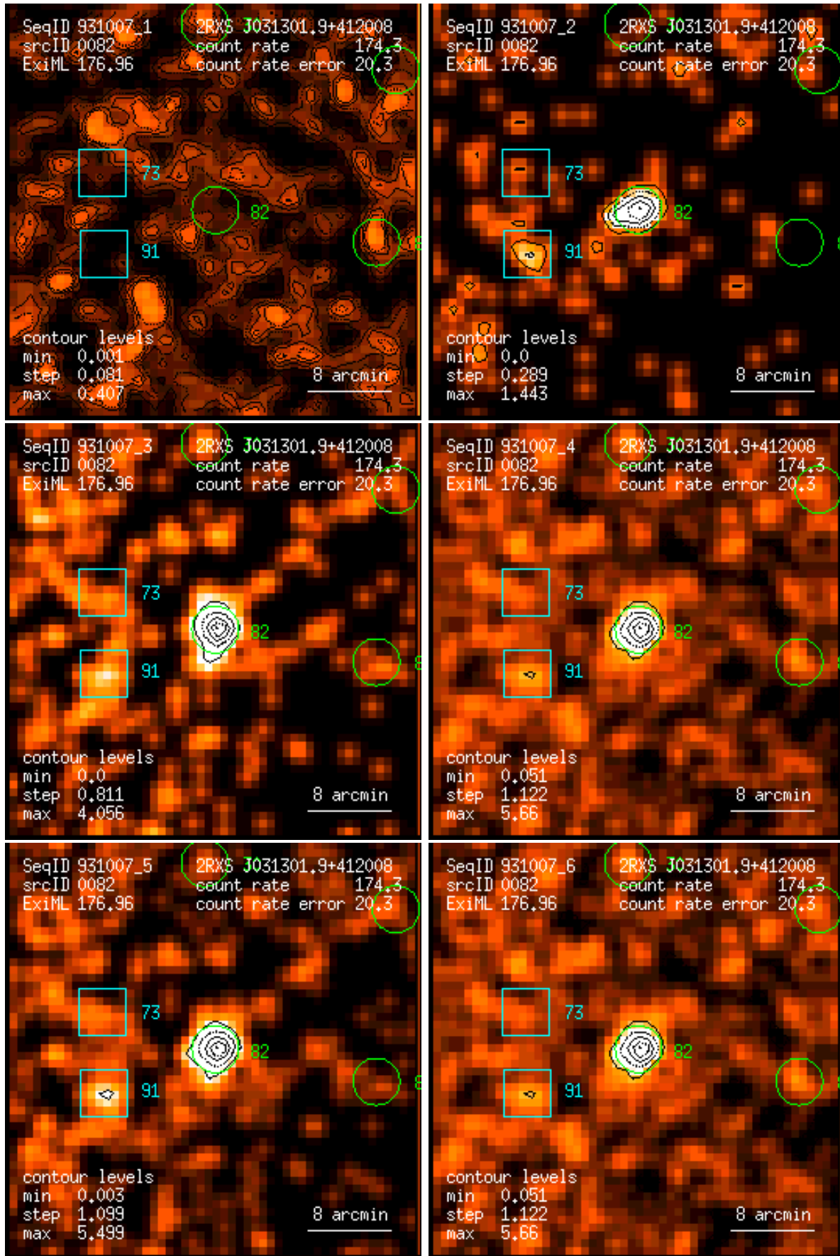
Figure 82: RASS 931007: detection 0082: band rate images, Gaussian filter: (1) PSPC channels 11 – 41, (2) 52 – 90, (3) 91 – 201, (4) 11 – 235, (5) 52 – 201, (6) 11 – 201. Broad band rates in counts/ks. Band rate contour levels in counts/ks/arcmin 2 .
