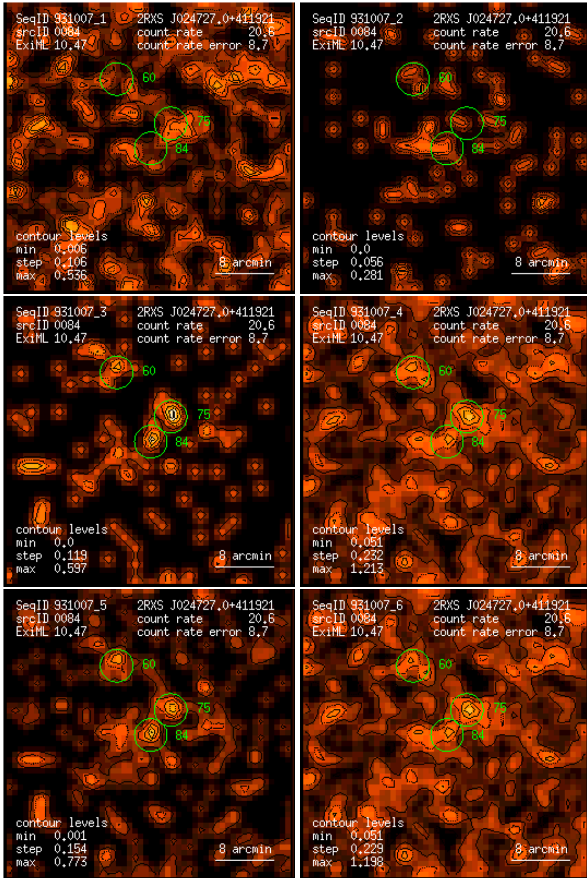
Figure 84: RASS 931007: detection 0084: band rate images, Gaussian filter: (1) PSPC channels 11 – 41, (2) 52 – 90, (3) 91 – 201, (4) 11 – 235, (5) 52 – 201, (6) 11 – 201. Broad band rates in counts/ks. Band rate contour levels in counts/ks/arcmin 2 .
