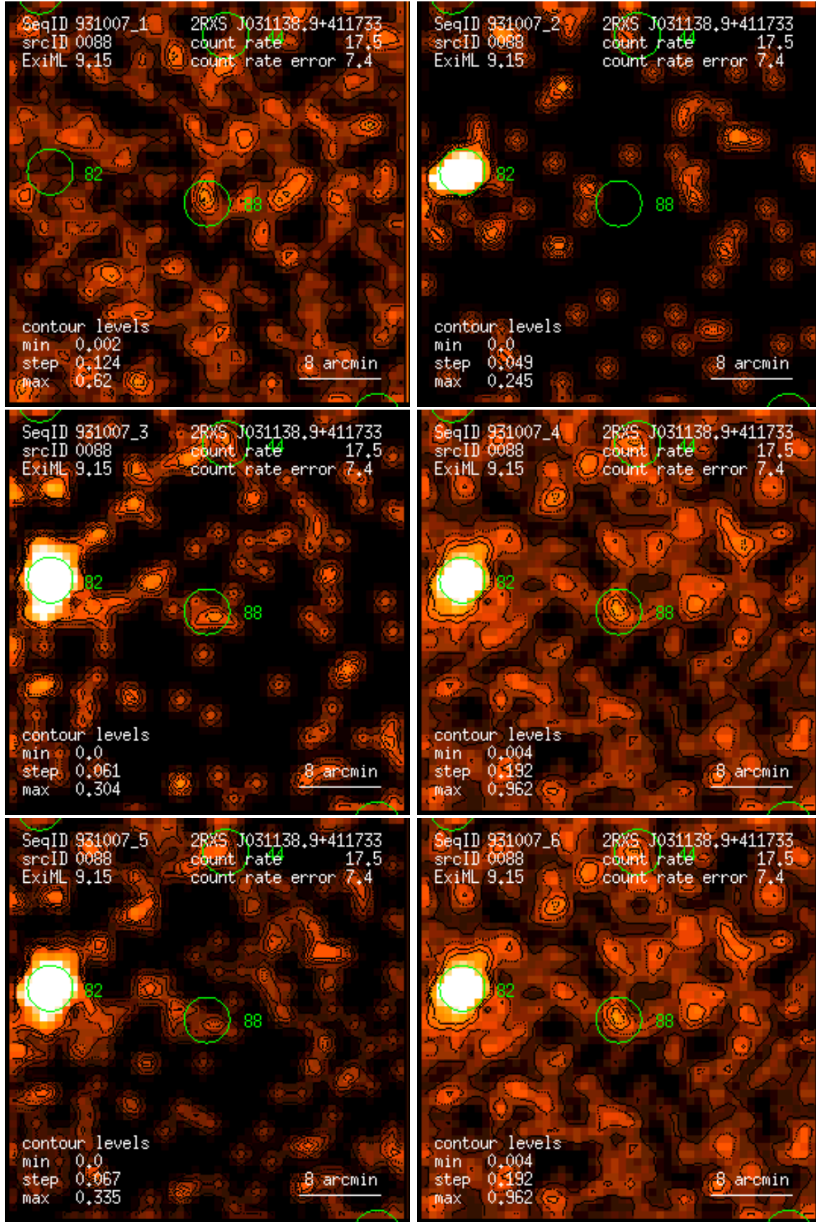
Figure 88: RASS 931007: detection 0088: band rate images, Gaussian filter: (1) PSPC channels 11 – 41, (2) 52 – 90, (3) 91 – 201, (4) 11 – 235, (5) 52 – 201, (6) 11 – 201. Broad band rates in counts/ks. Band rate contour levels in counts/ks/arcmin 2 .
