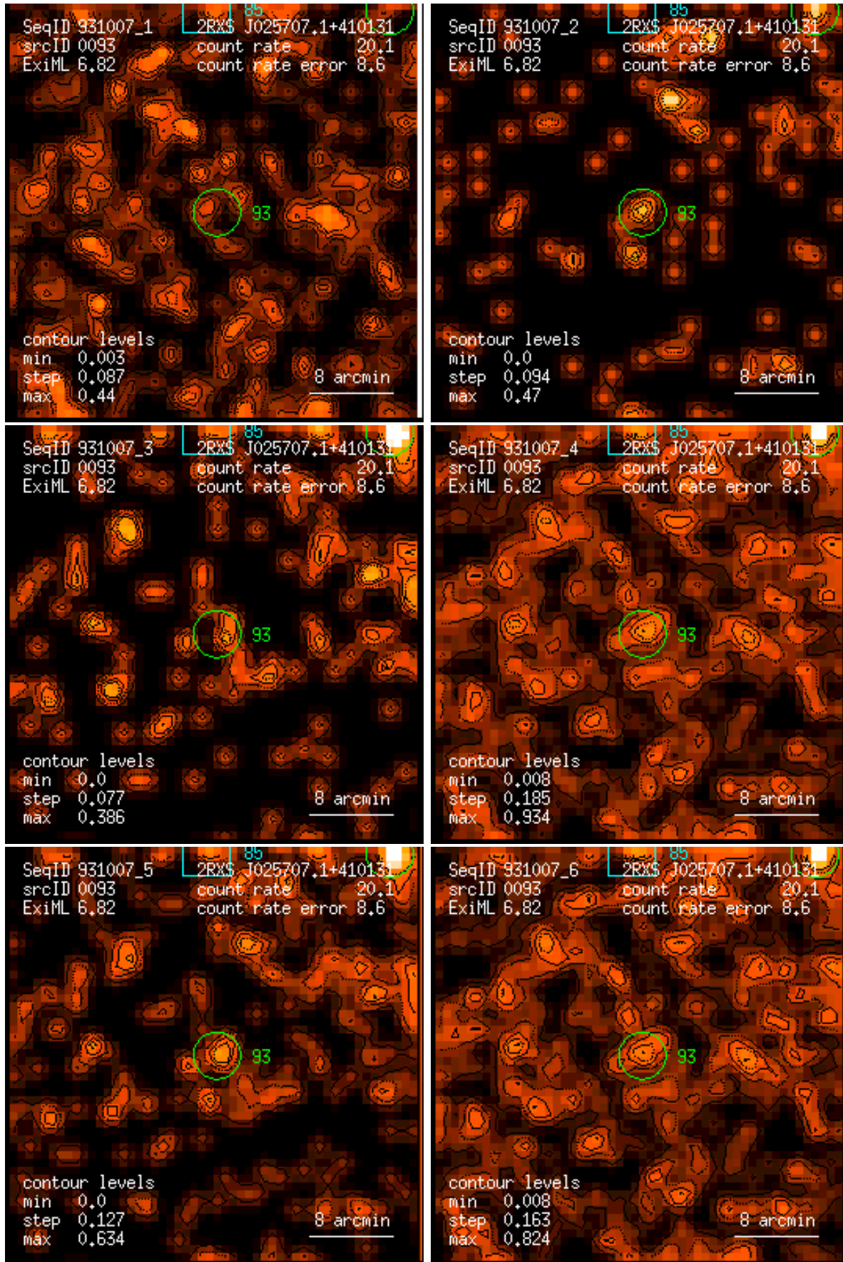
Figure 93: RASS 931007: detection 0093: band rate images, Gaussian filter: (1) PSPC channels 11 – 41, (2) 52 – 90, (3) 91 – 201, (4) 11 – 235, (5) 52 – 201, (6) 11 – 201. Broad band rates in counts/ks. Band rate contour levels in counts/ks/arcmin 2 .
